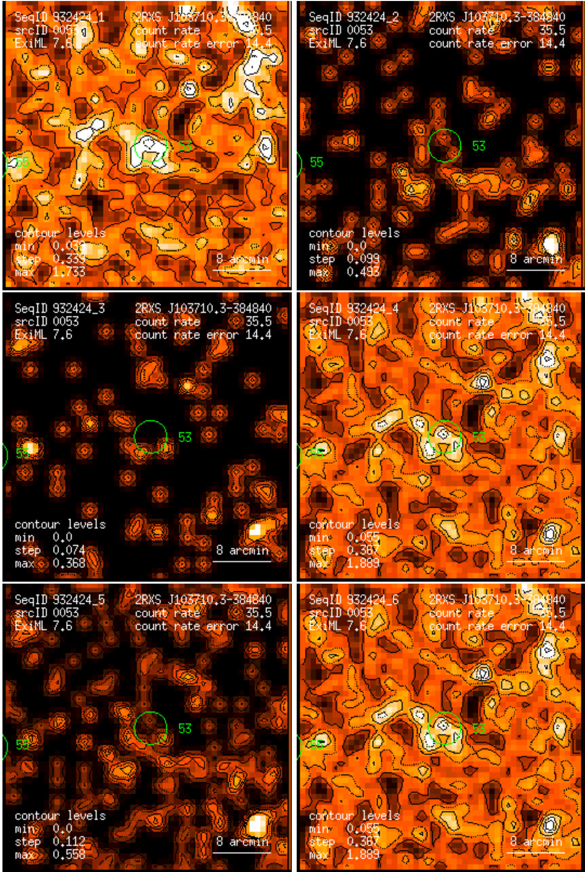
Figure 53: RASS 932424: detection 0053: band rate images, Gaussian filter: (1) PSPC channels 11 – 41, (2) 52 – 90, (3) 91 – 201, (4) 11 – 235, (5) 52 – 201, (6) 11 – 201. Broad band rates in counts/ks. Band rate contour levels in counts/ks/arcmin 2 .
