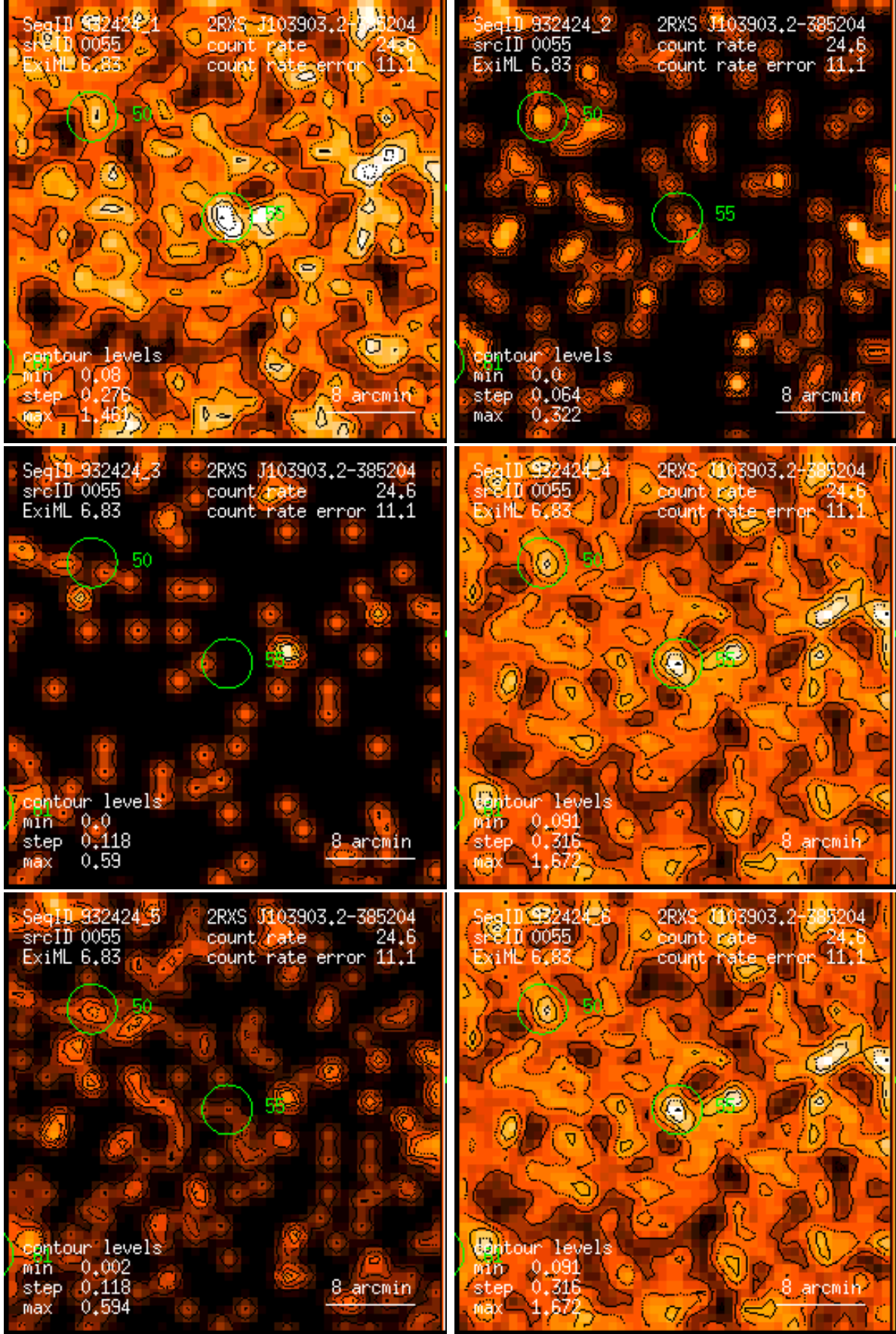
Figure 55: RASS 932424: detection 0055: band rate images, Gaussian filter: (1) PSPC channels 11 – 41, (2) 52 – 90, (3) 91 – 201, (4) 11 – 235, (5) 52 – 201, (6) 11 – 201. Broad band rates in counts/ks. Band rate contour levels in counts/ks/arcmin 2 .
