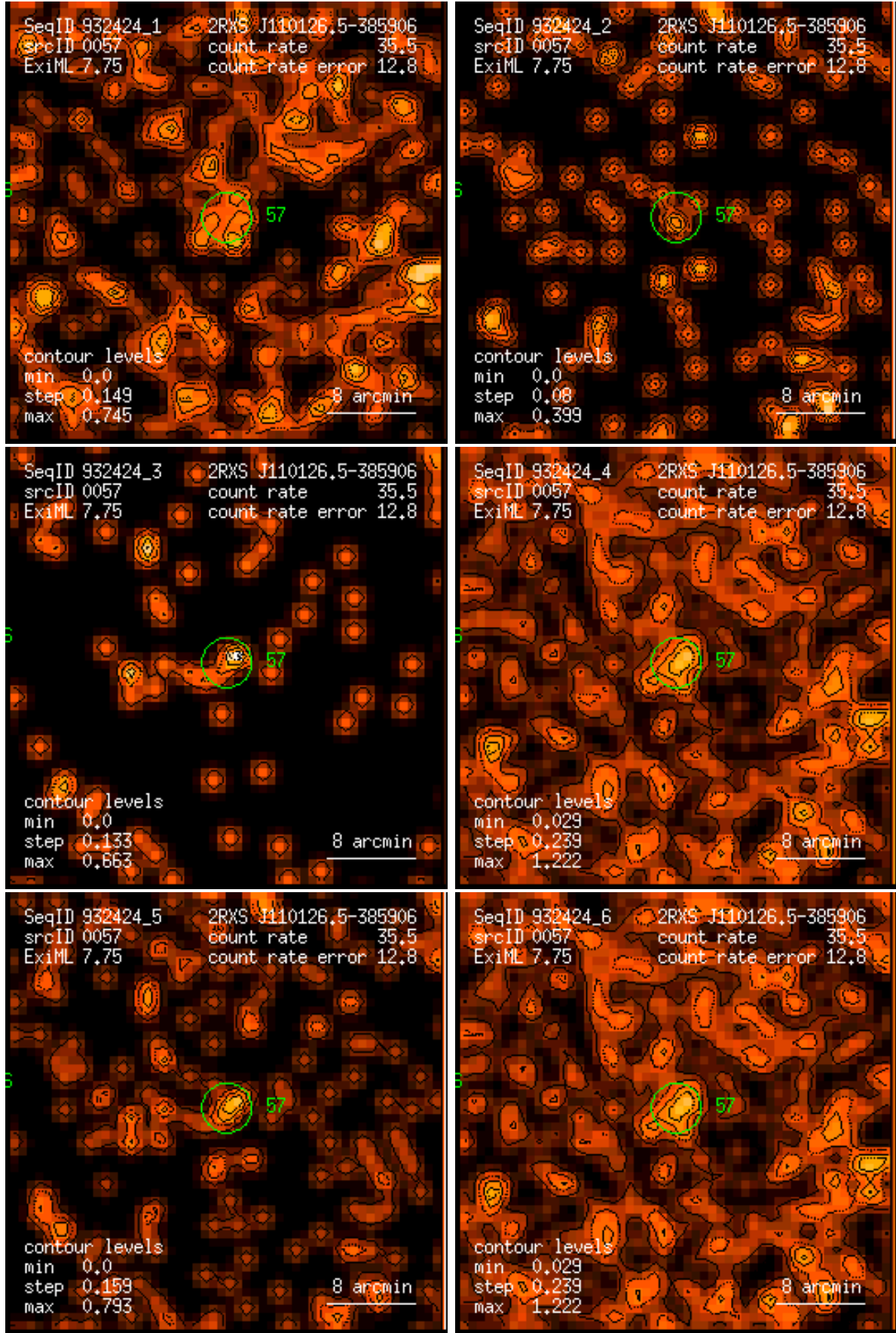
Figure 57: RASS 932424: detection 0057: band rate images, Gaussian filter: (1) PSPC channels 11 – 41, (2) 52 – 90, (3) 91 – 201, (4) 11 – 235, (5) 52 – 201, (6) 11 – 201. Broad band rates in counts/ks. Band rate contour levels in counts/ks/arcmin 2 .
