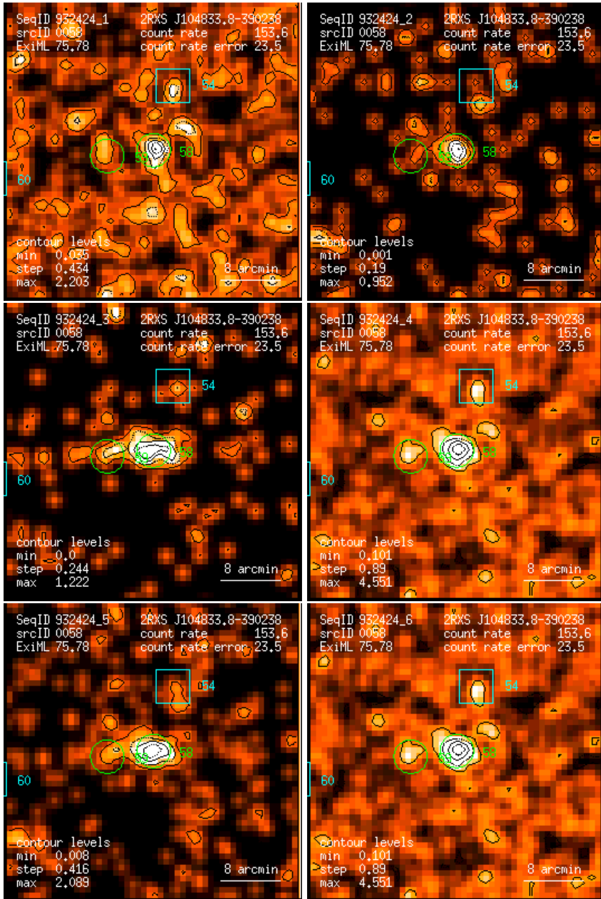
Figure 58: RASS 932424: detection 0058: band rate images, Gaussian filter: (1) PSPC channels 11 – 41, (2) 52 – 90, (3) 91 – 201, (4) 11 – 235, (5) 52 – 201, (6) 11 – 201. Broad band rates in counts/ks. Band rate contour levels in counts/ks/arcmin 2 .
