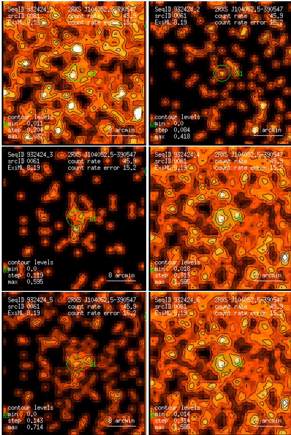
Figure 61: RASS 932424: detection 0061: band rate images, Gaussian filter: (1) PSPC channels 11 – 41, (2) 52 – 90, (3) 91 – 201, (4) 11 – 235, (5) 52 – 201, (6) 11 – 201. Broad band rates in counts/ks. Band rate contour levels in counts/ks/arcmin 2 .
