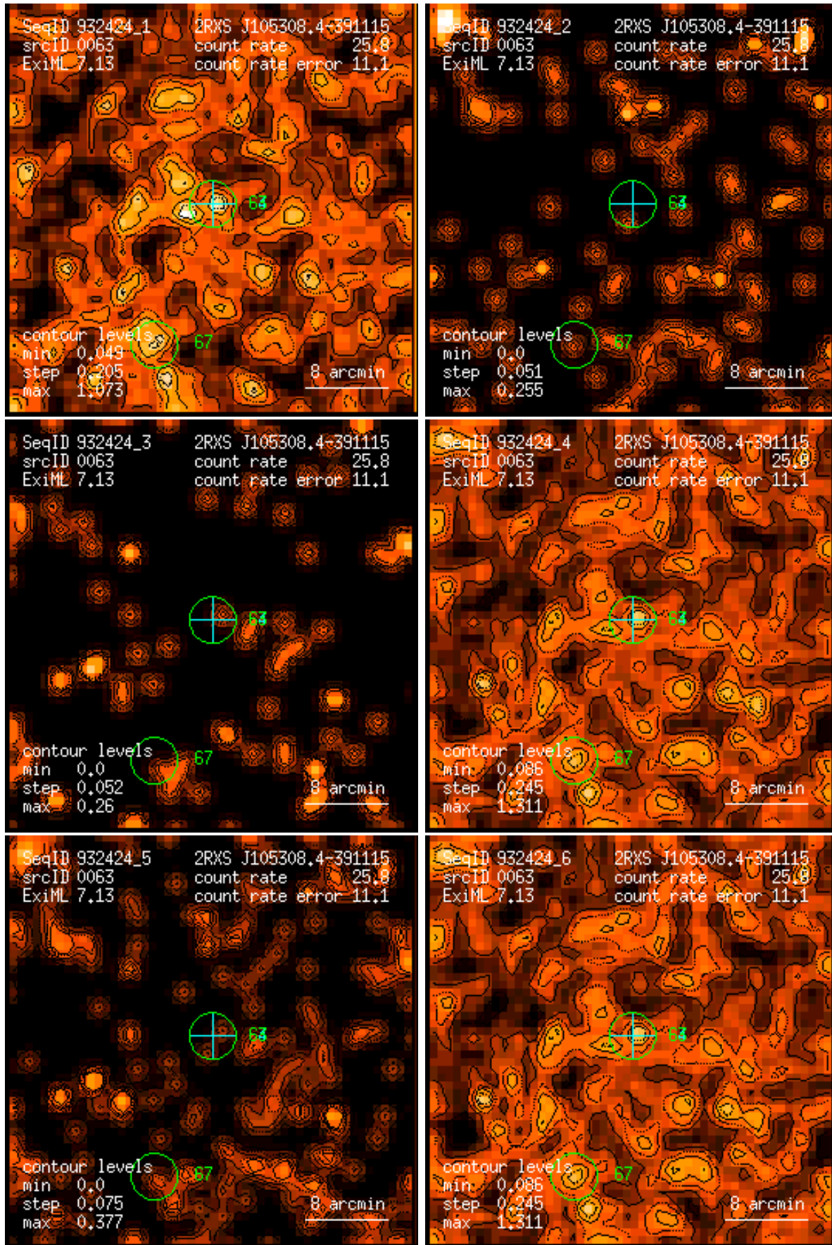
Figure 63: RASS 932424: detection 0063: band rate images, Gaussian filter: (1) PSPC channels 11 – 41, (2) 52 – 90, (3) 91 – 201, (4) 11 – 235, (5) 52 – 201, (6) 11 – 201. Broad band rates in counts/ks. Band rate contour levels in counts/ks/arcmin 2 .
