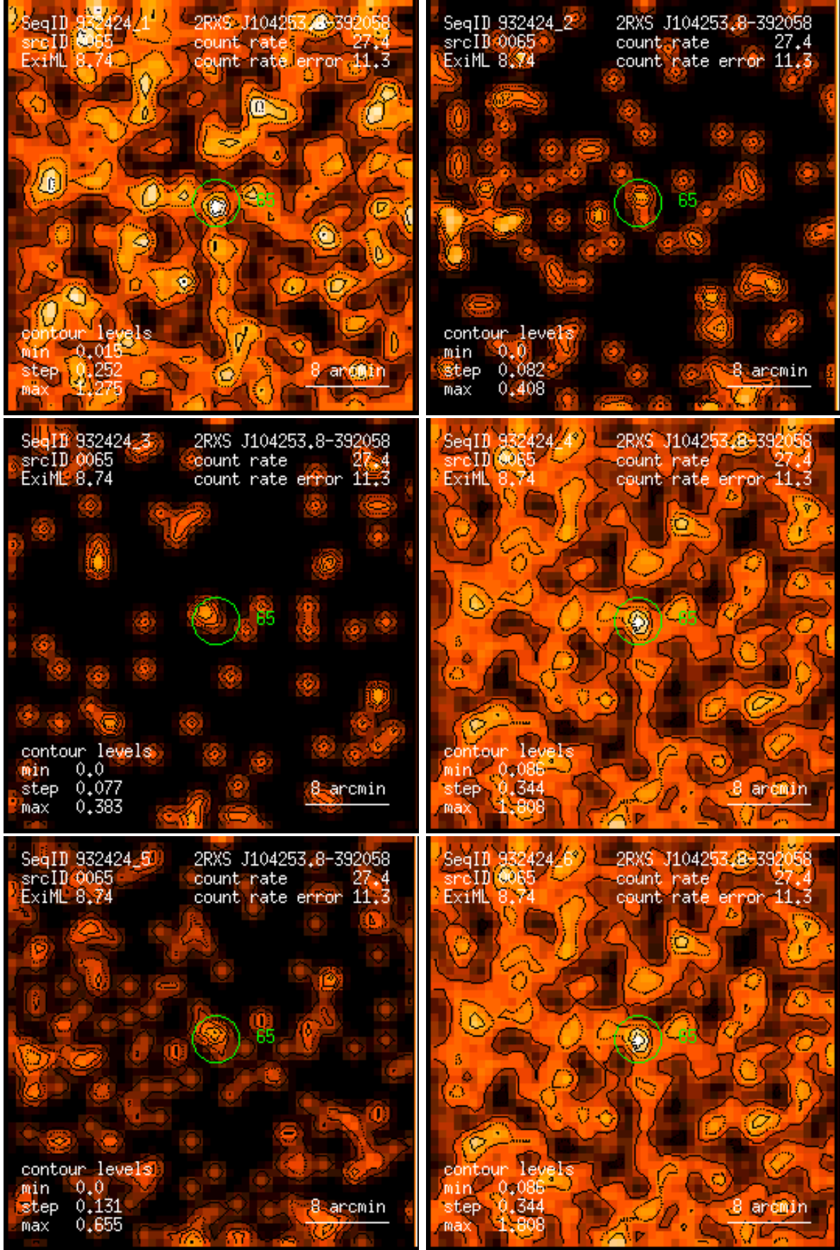
Figure 65: RASS 932424: detection 0065: band rate images, Gaussian filter: (1) PSPC channels 11 – 41, (2) 52 – 90, (3) 91 – 201, (4) 11 – 235, (5) 52 – 201, (6) 11 – 201. Broad band rates in counts/ks. Band rate contour levels in counts/ks/arcmin 2 .
