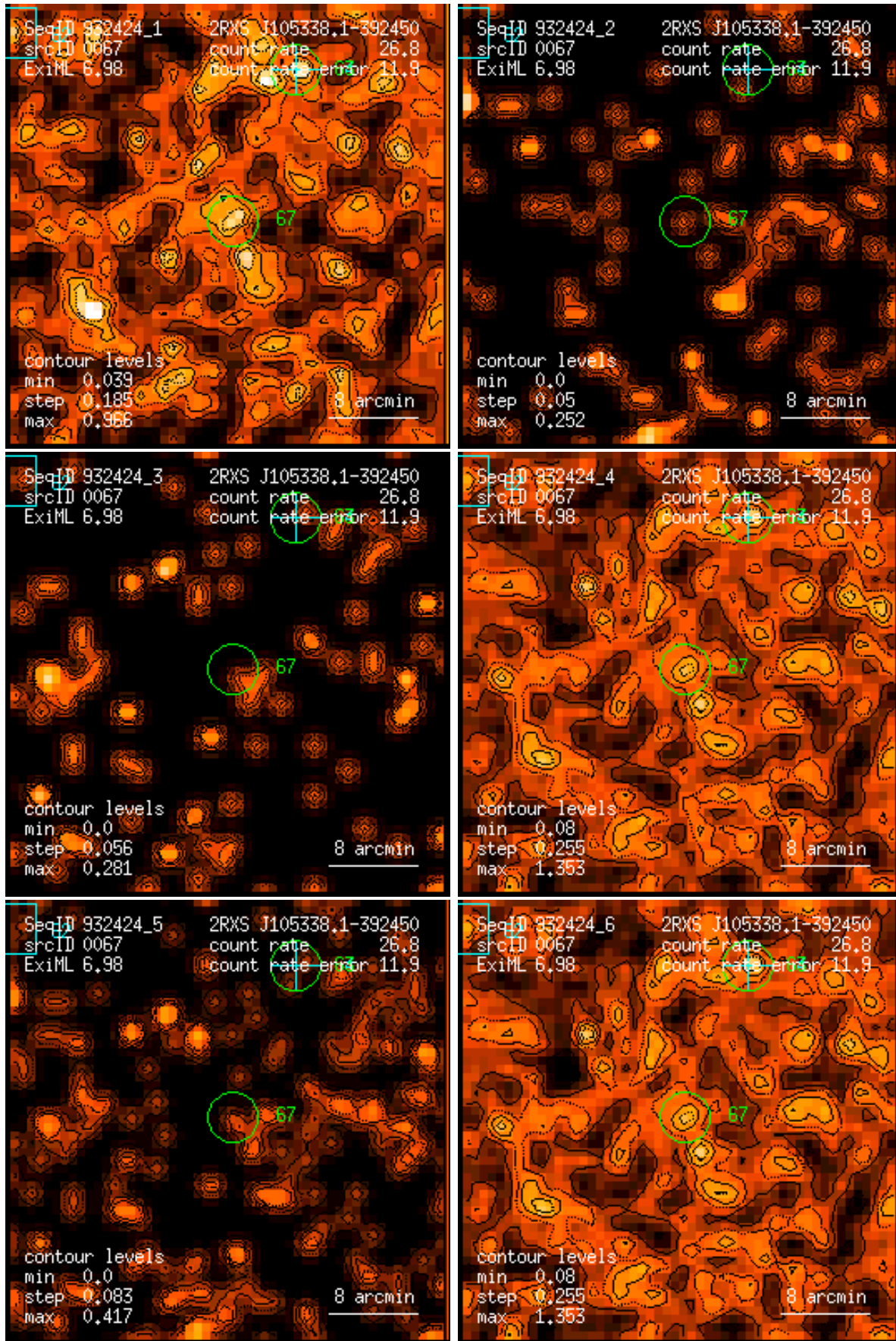
Figure 67: RASS 932424: detection 0067: band rate images, Gaussian filter: (1) PSPC channels 11 – 41, (2) 52 – 90, (3) 91 – 201, (4) 11 – 235, (5) 52 – 201, (6) 11 – 201. Broad band rates in counts/ks. Band rate contour levels in counts/ks/arcmin 2 .
