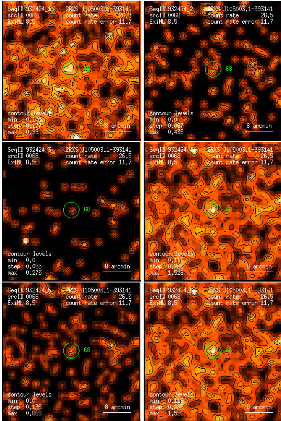
Figure 68: RASS 932424: detection 0068: band rate images, Gaussian filter: (1) PSPC channels 11 – 41, (2) 52 – 90, (3) 91 – 201, (4) 11 – 235, (5) 52 – 201, (6) 11 – 201. Broad band rates in counts/ks. Band rate contour levels in counts/ks/arcmin 2 .
