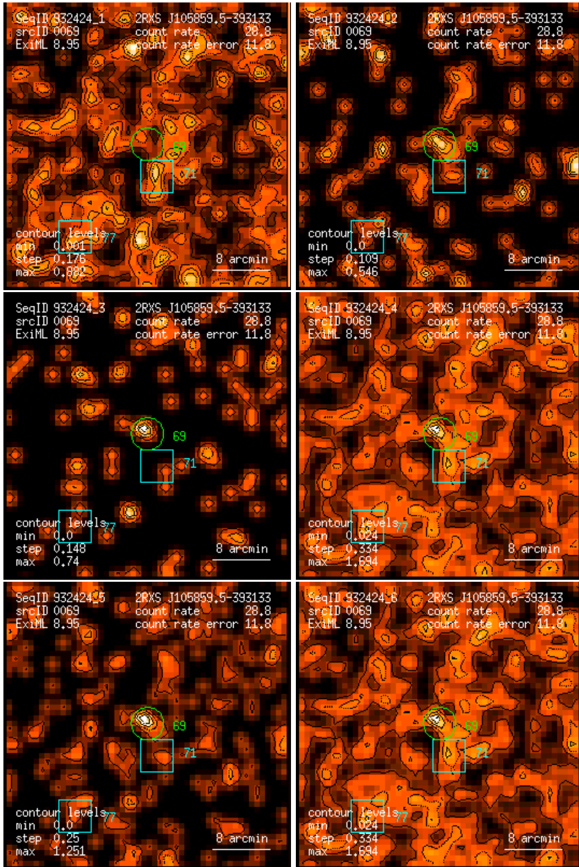
Figure 69: RASS 932424: detection 0069: band rate images, Gaussian filter: (1) PSPC channels 11 – 41, (2) 52 – 90, (3) 91 – 201, (4) 11 – 235, (5) 52 – 201, (6) 11 – 201. Broad band rates in counts/ks. Band rate contour levels in counts/ks/arcmin 2 .
