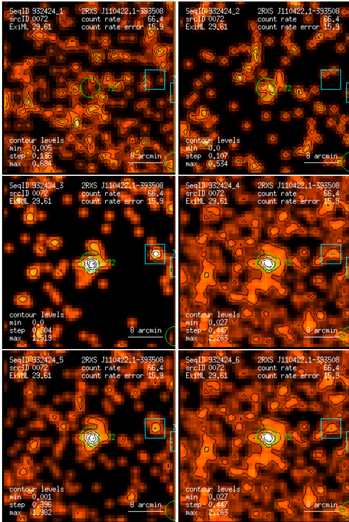
Figure 72: RASS 932424: detection 0072: band rate images, Gaussian filter: (1) PSPC channels 11 – 41, (2) 52 – 90, (3) 91 – 201, (4) 11 – 235, (5) 52 – 201, (6) 11 – 201. Broad band rates in counts/ks. Band rate contour levels in counts/ks/arcmin 2 .
