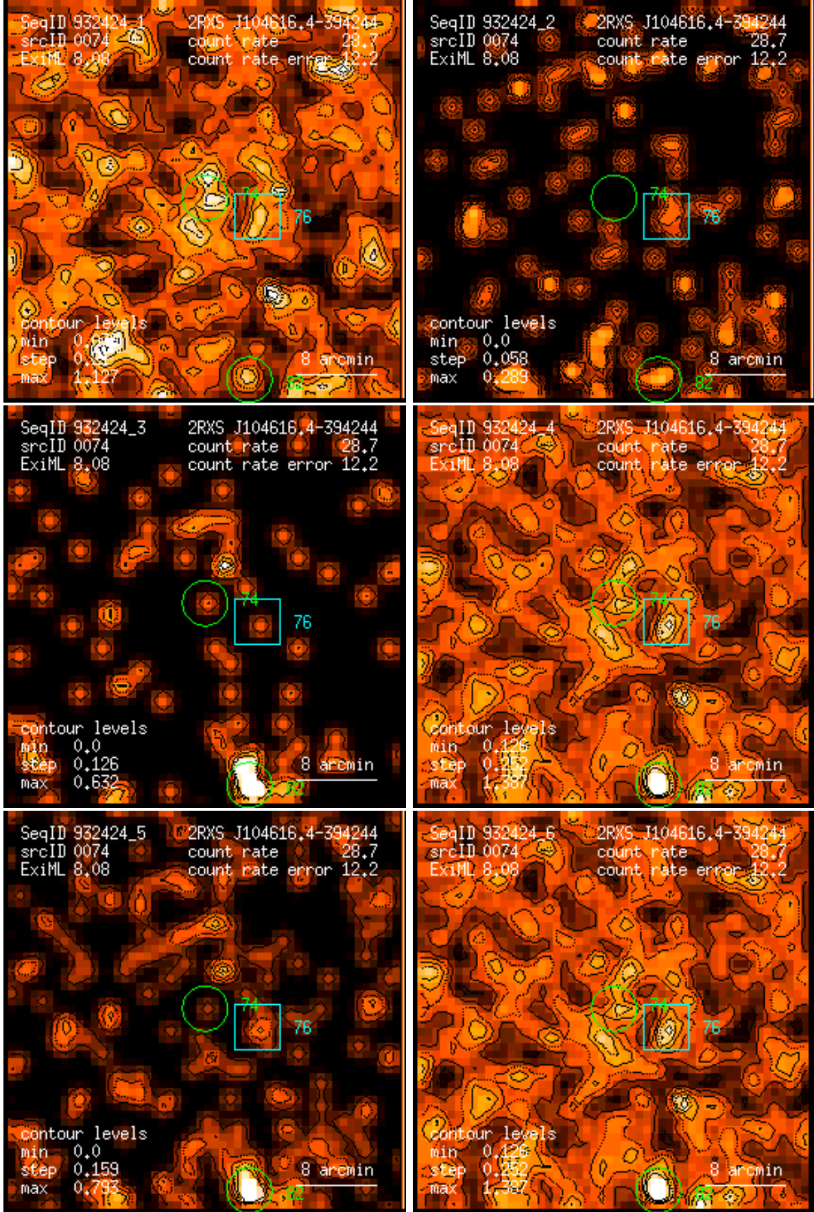
Figure 74: RASS 932424: detection 0074: band rate images, Gaussian filter: (1) PSPC channels 11 – 41, (2) 52 – 90, (3) 91 – 201, (4) 11 – 235, (5) 52 – 201, (6) 11 – 201. Broad band rates in counts/ks. Band rate contour levels in counts/ks/arcmin 2 .
