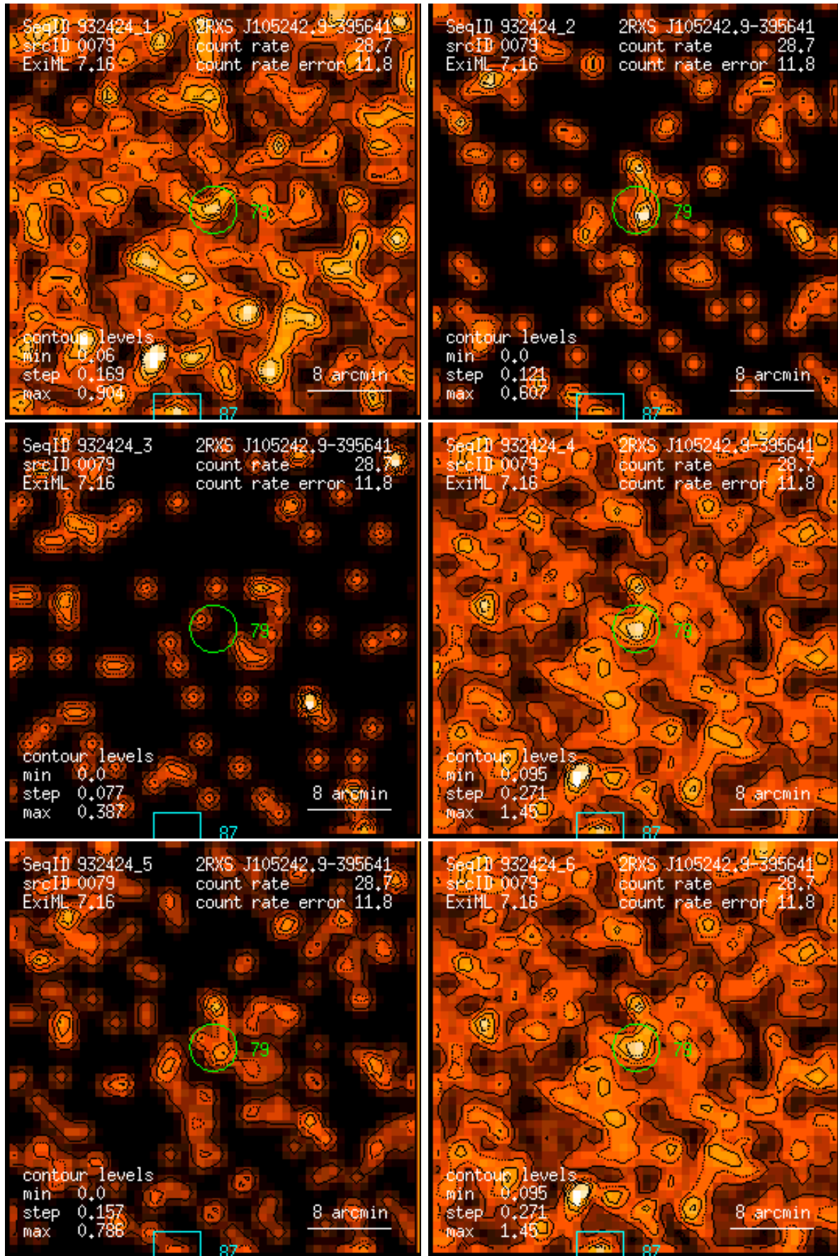
Figure 79: RASS 932424: detection 0079: band rate images, Gaussian filter: (1) PSPC channels 11 – 41, (2) 52 – 90, (3) 91 – 201, (4) 11 – 235, (5) 52 – 201, (6) 11 – 201. Broad band rates in counts/ks. Band rate contour levels in counts/ks/arcmin 2 .
