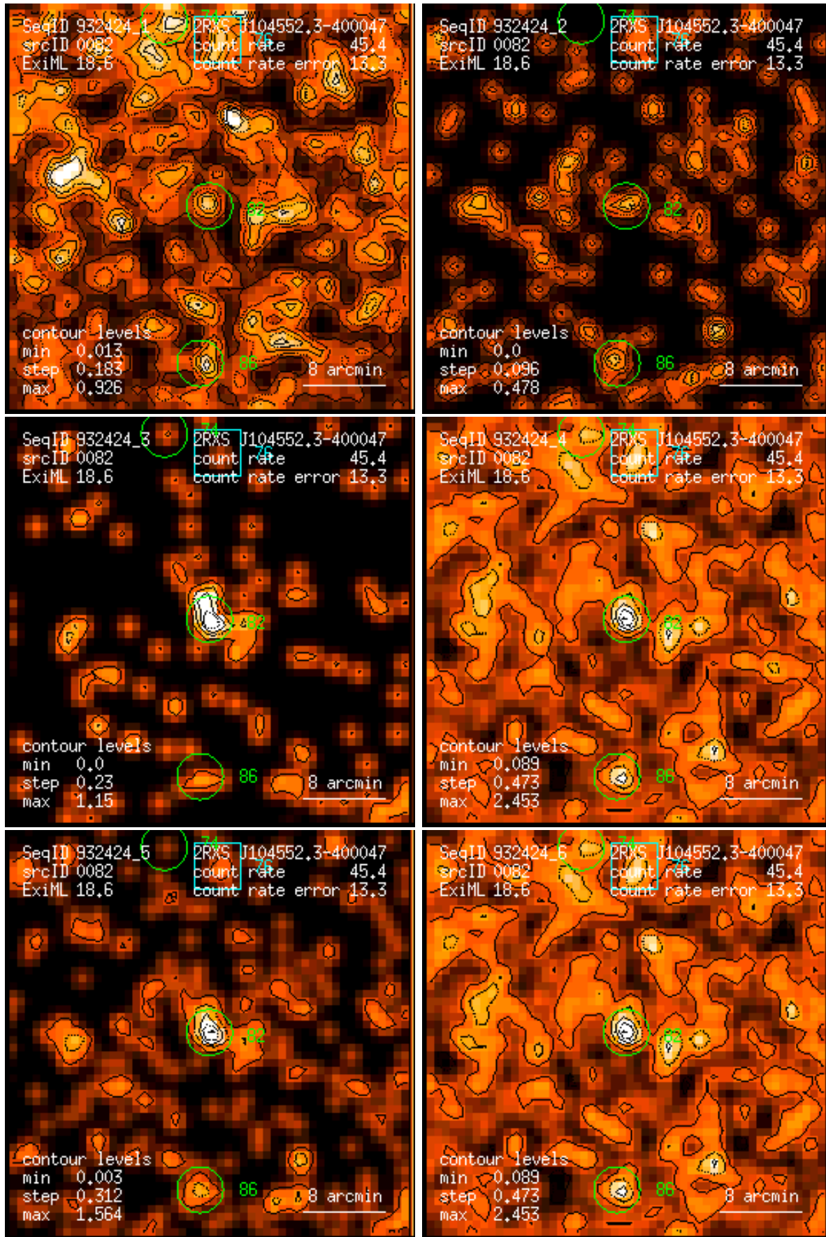
Figure 82: RASS 932424: detection 0082: band rate images, Gaussian filter: (1) PSPC channels 11 – 41, (2) 52 – 90, (3) 91 – 201, (4) 11 – 235, (5) 52 – 201, (6) 11 – 201. Broad band rates in counts/ks. Band rate contour levels in counts/ks/arcmin 2 .
