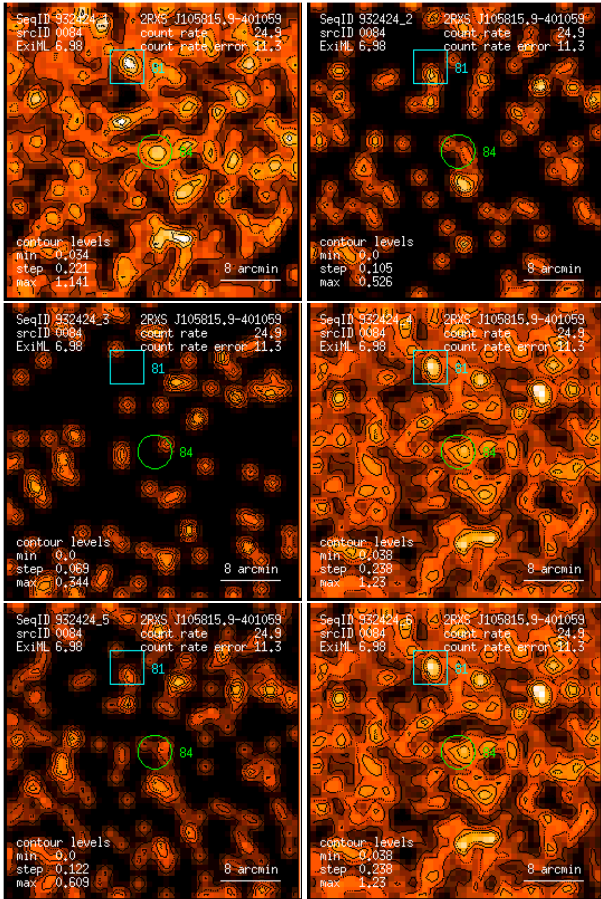
Figure 84: RASS 932424: detection 0084: band rate images, Gaussian filter: (1) PSPC channels 11 – 41, (2) 52 – 90, (3) 91 – 201, (4) 11 – 235, (5) 52 – 201, (6) 11 – 201. Broad band rates in counts/ks. Band rate contour levels in counts/ks/arcmin 2 .
