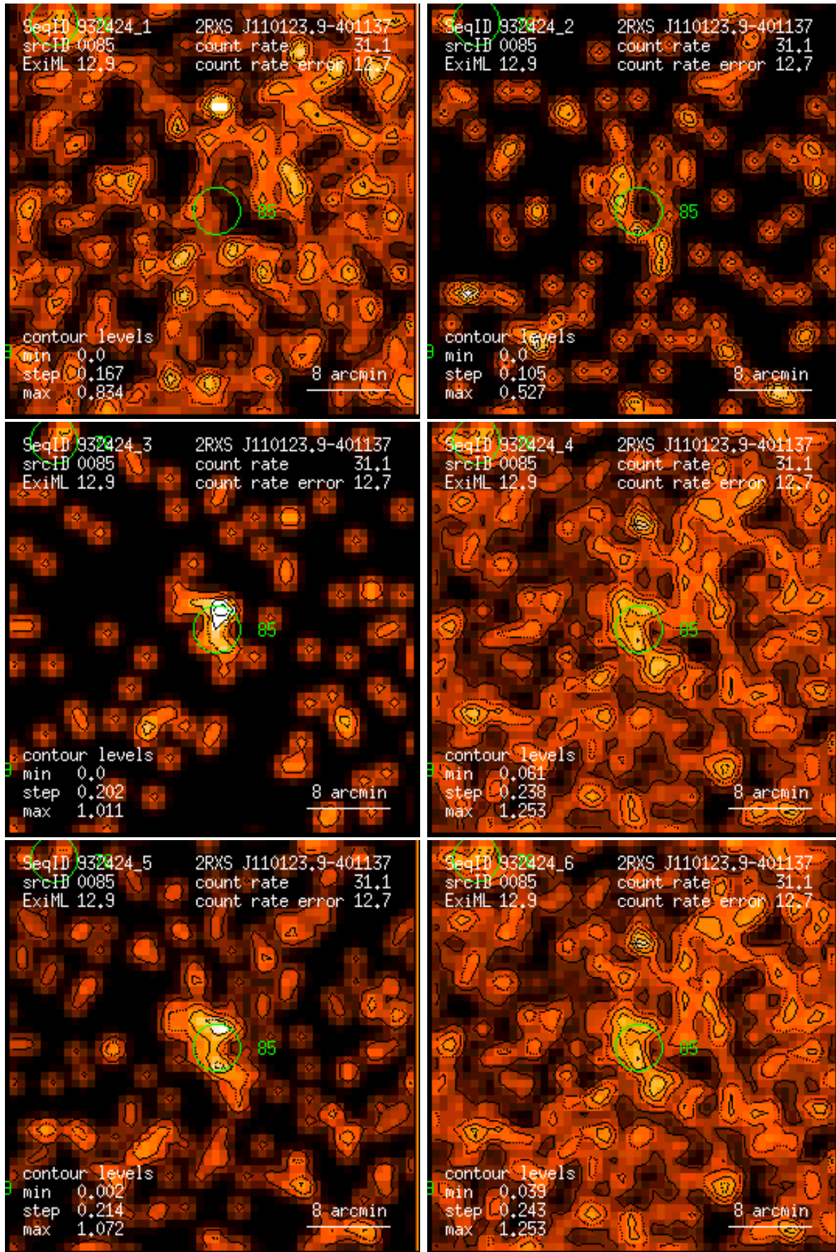
Figure 85: RASS 932424: detection 0085: band rate images, Gaussian filter: (1) PSPC channels 11 – 41, (2) 52 – 90, (3) 91 – 201, (4) 11 – 235, (5) 52 – 201, (6) 11 – 201. Broad band rates in counts/ks. Band rate contour levels in counts/ks/arcmin 2 .
