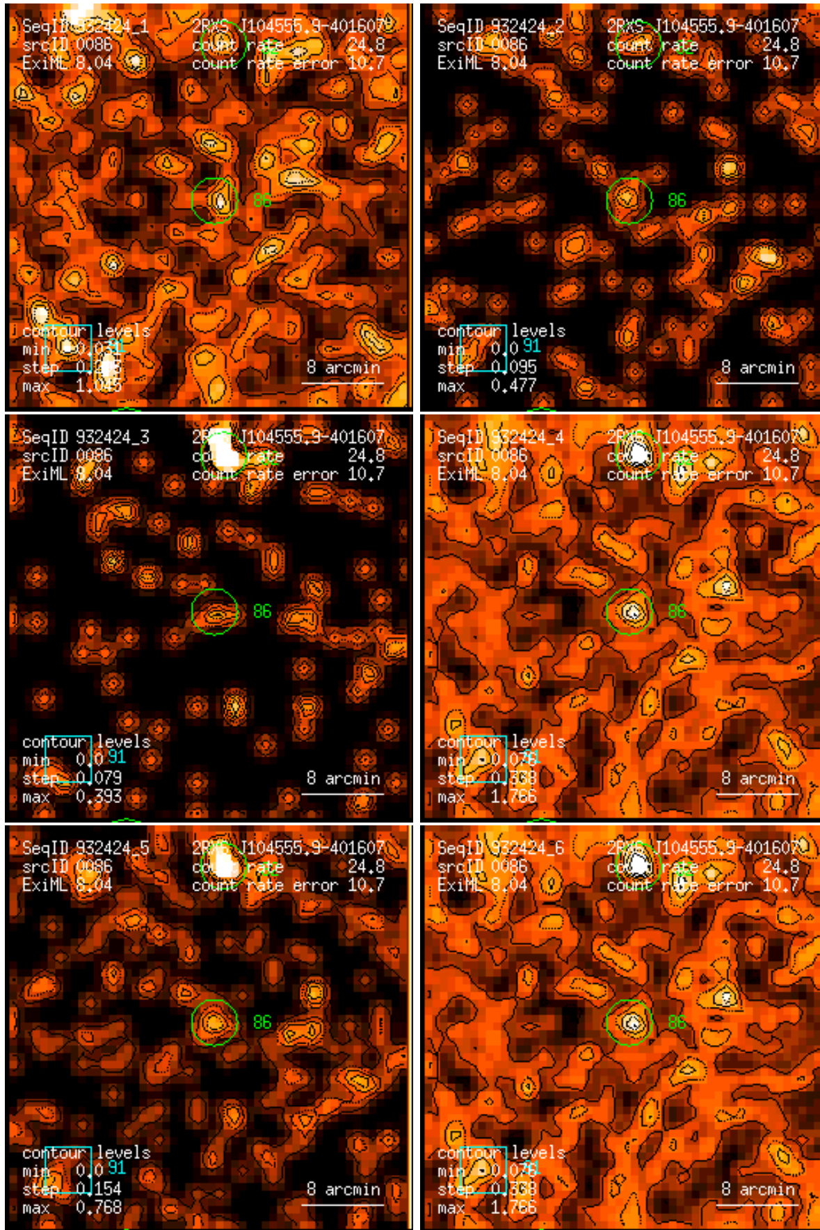
Figure 86: RASS 932424: detection 0086: band rate images, Gaussian filter: (1) PSPC channels 11 – 41, (2) 52 – 90, (3) 91 – 201, (4) 11 – 235, (5) 52 – 201, (6) 11 – 201. Broad band rates in counts/ks. Band rate contour levels in counts/ks/arcmin 2 .
