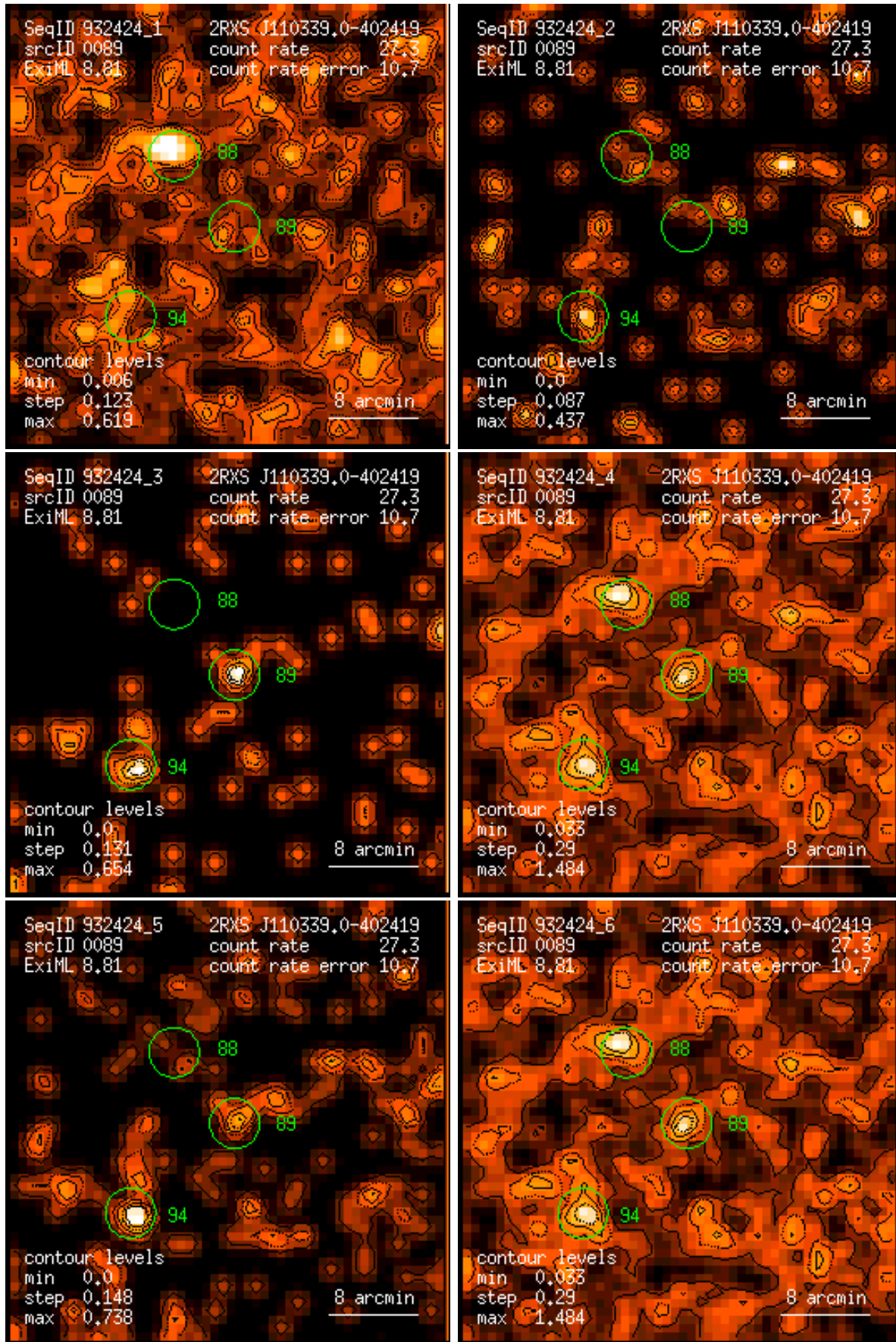
Figure 89: RASS 932424: detection 0089: band rate images, Gaussian filter: (1) PSPC channels 11 – 41, (2) 52 – 90, (3) 91 – 201, (4) 11 – 235, (5) 52 – 201, (6) 11 – 201. Broad band rates in counts/ks. Band rate contour levels in counts/ks/arcmin 2 .
