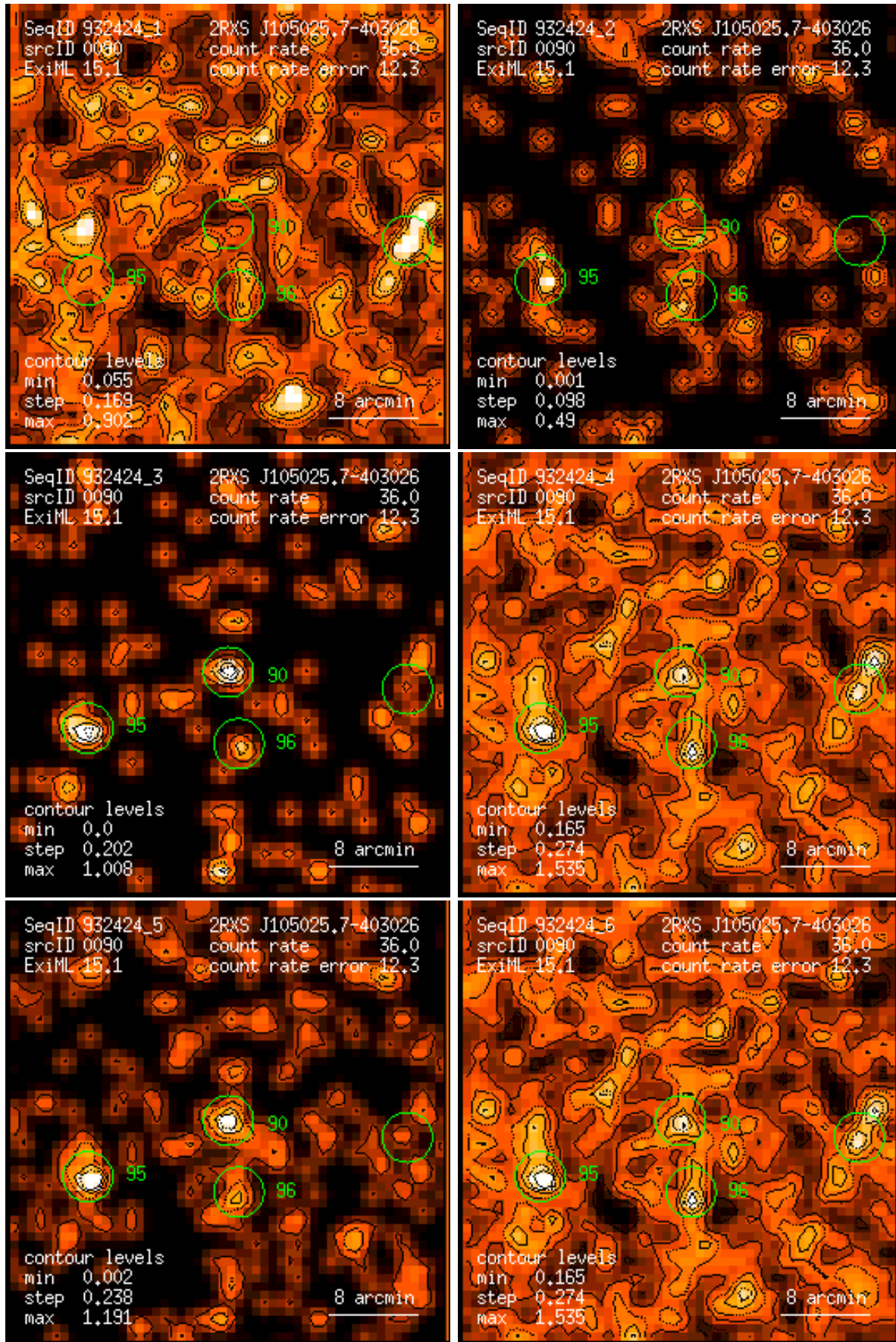
Figure 90: RASS 932424: detection 0090: band rate images, Gaussian filter: (1) PSPC channels 11 – 41, (2) 52 – 90, (3) 91 – 201, (4) 11 – 235, (5) 52 – 201, (6) 11 – 201. Broad band rates in counts/ks. Band rate contour levels in counts/ks/arcmin 2 .
