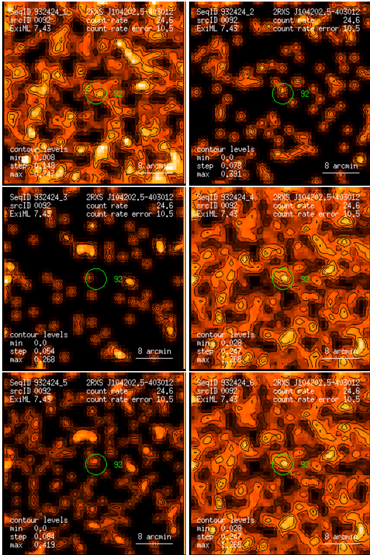
Figure 92: RASS 932424: detection 0092: band rate images, Gaussian filter: (1) PSPC channels 11 – 41, (2) 52 – 90, (3) 91 – 201, (4) 11 – 235, (5) 52 – 201, (6) 11 – 201. Broad band rates in counts/ks. Band rate contour levels in counts/ks/arcmin 2 .
