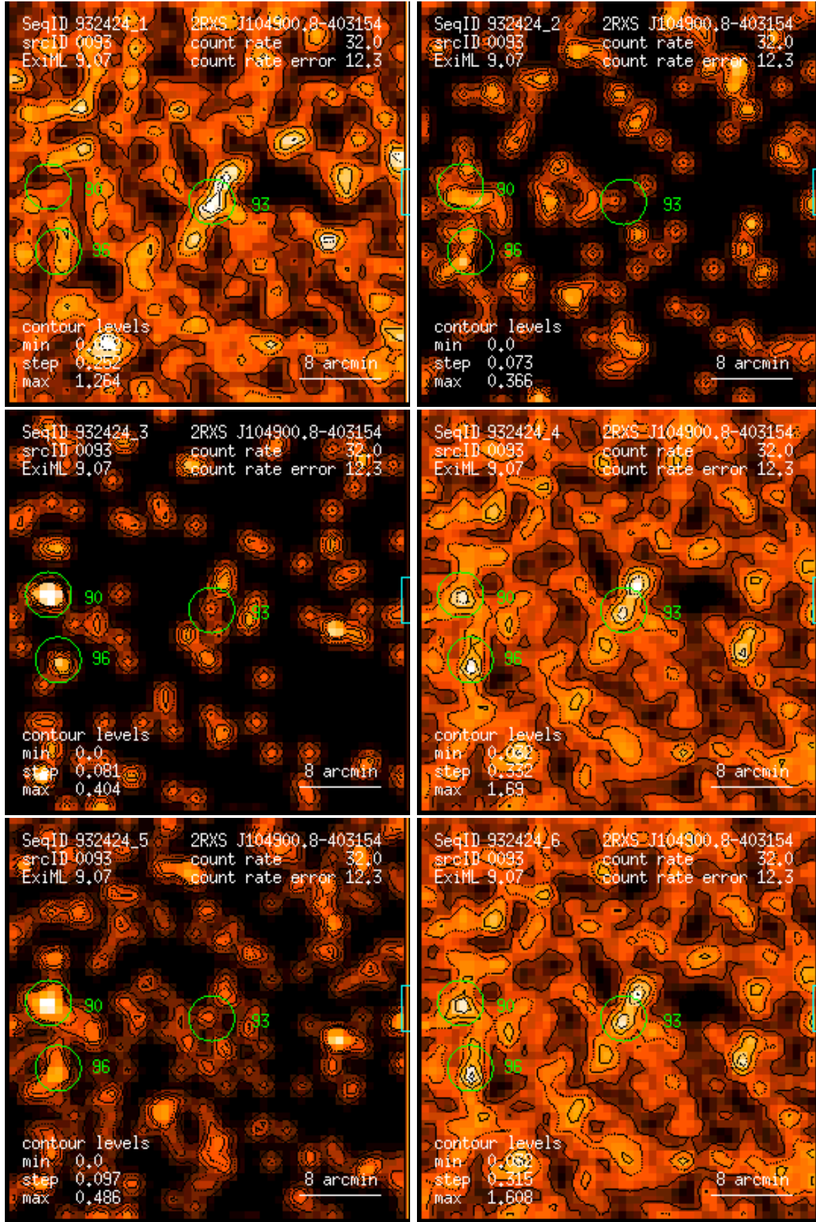
Figure 93: RASS 932424: detection 0093: band rate images, Gaussian filter: (1) PSPC channels 11 – 41, (2) 52 – 90, (3) 91 – 201, (4) 11 – 235, (5) 52 – 201, (6) 11 – 201. Broad band rates in counts/ks. Band rate contour levels in counts/ks/arcmin 2 .
