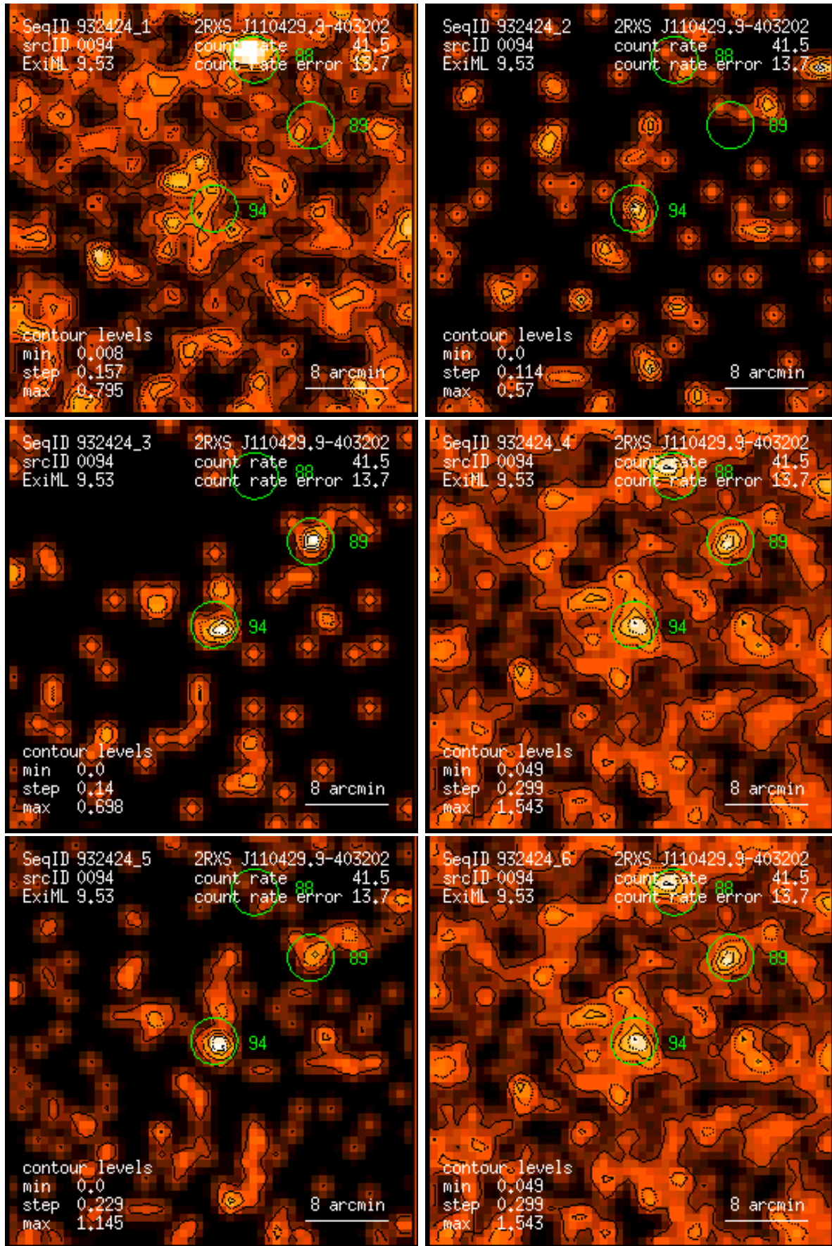
Figure 94: RASS 932424: detection 0094: band rate images, Gaussian filter: (1) PSPC channels 11 – 41, (2) 52 – 90, (3) 91 – 201, (4) 11 – 235, (5) 52 – 201, (6) 11 – 201. Broad band rates in counts/ks. Band rate contour levels in counts/ks/arcmin 2 .
