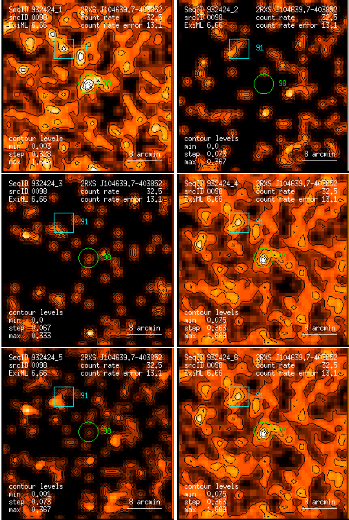
Figure 98: RASS 932424: detection 0098: band rate images, Gaussian filter: (1) PSPC channels 11 – 41, (2) 52 – 90, (3) 91 – 201, (4) 11 – 235, (5) 52 – 201, (6) 11 – 201. Broad band rates in counts/ks. Band rate contour levels in counts/ks/arcmin 2 .
