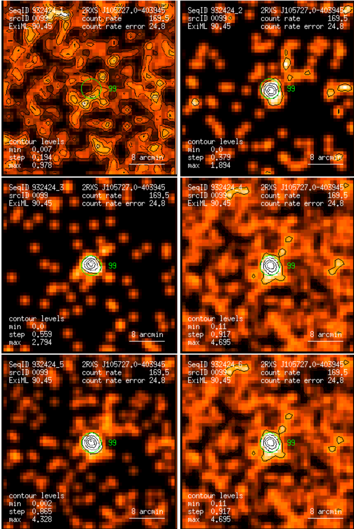
Figure 99: RASS 932424: detection 0099: band rate images, Gaussian filter: (1) PSPC channels 11 – 41, (2) 52 – 90, (3) 91 – 201, (4) 11 – 235, (5) 52 – 201, (6) 11 – 201. Broad band rates in counts/ks. Band rate contour levels in counts/ks/arcmin 2 .
