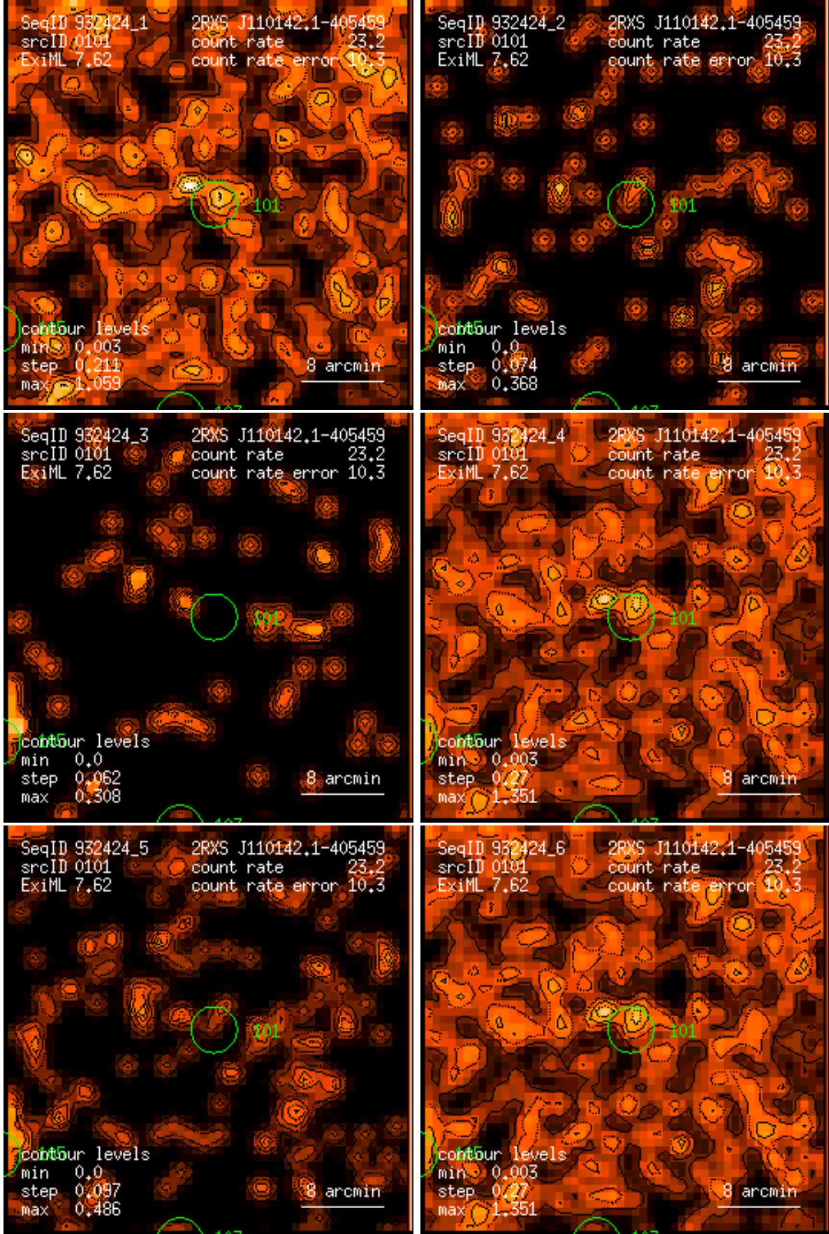
Figure 101: RASS 932424: detection 0101: band rate images, Gaussian filter: (1) PSPC channels 11 – 41, (2) 52 – 90, (3) 91 – 201, (4) 11 – 235, (5) 52 – 201, (6) 11 – 201. Broad band rates in counts/ks. Band rate contour levels in counts/ks/arcmin 2 .
