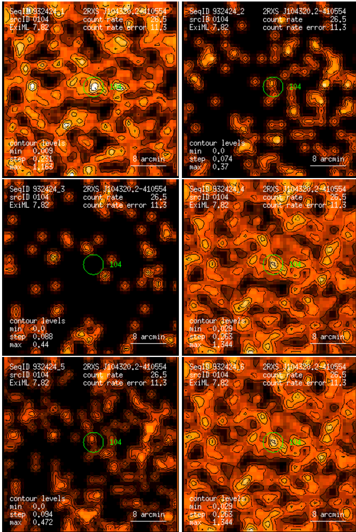
Figure 104: RASS 932424: detection 0104: band rate images, Gaussian filter: (1) PSPC channels 11 – 41, (2) 52 – 90, (3) 91 – 201, (4) 11 – 235, (5) 52 – 201, (6) 11 – 201. Broad band rates in counts/ks. Band rate contour levels in counts/ks/arcmin 2 .
