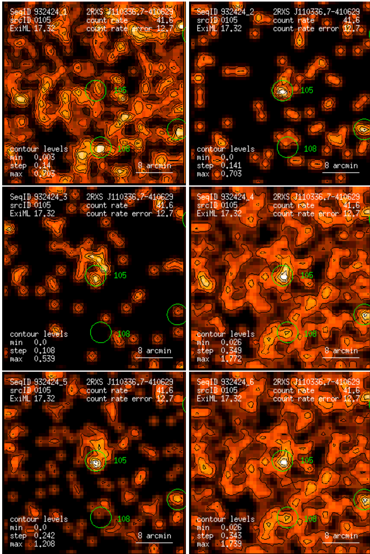
Figure 105: RASS 932424: detection 0105: band rate images, Gaussian filter: (1) PSPC channels 11 – 41, (2) 52 – 90, (3) 91 – 201, (4) 11 – 235, (5) 52 – 201, (6) 11 – 201. Broad band rates in counts/ks. Band rate contour levels in counts/ks/arcmin 2 .
