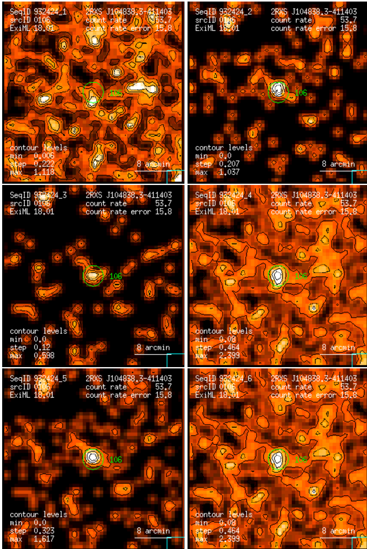
Figure 106: RASS 932424: detection 0106: band rate images, Gaussian filter: (1) PSPC channels 11 – 41, (2) 52 – 90, (3) 91 – 201, (4) 11 – 235, (5) 52 – 201, (6) 11 – 201. Broad band rates in counts/ks. Band rate contour levels in counts/ks/arcmin 2 .
