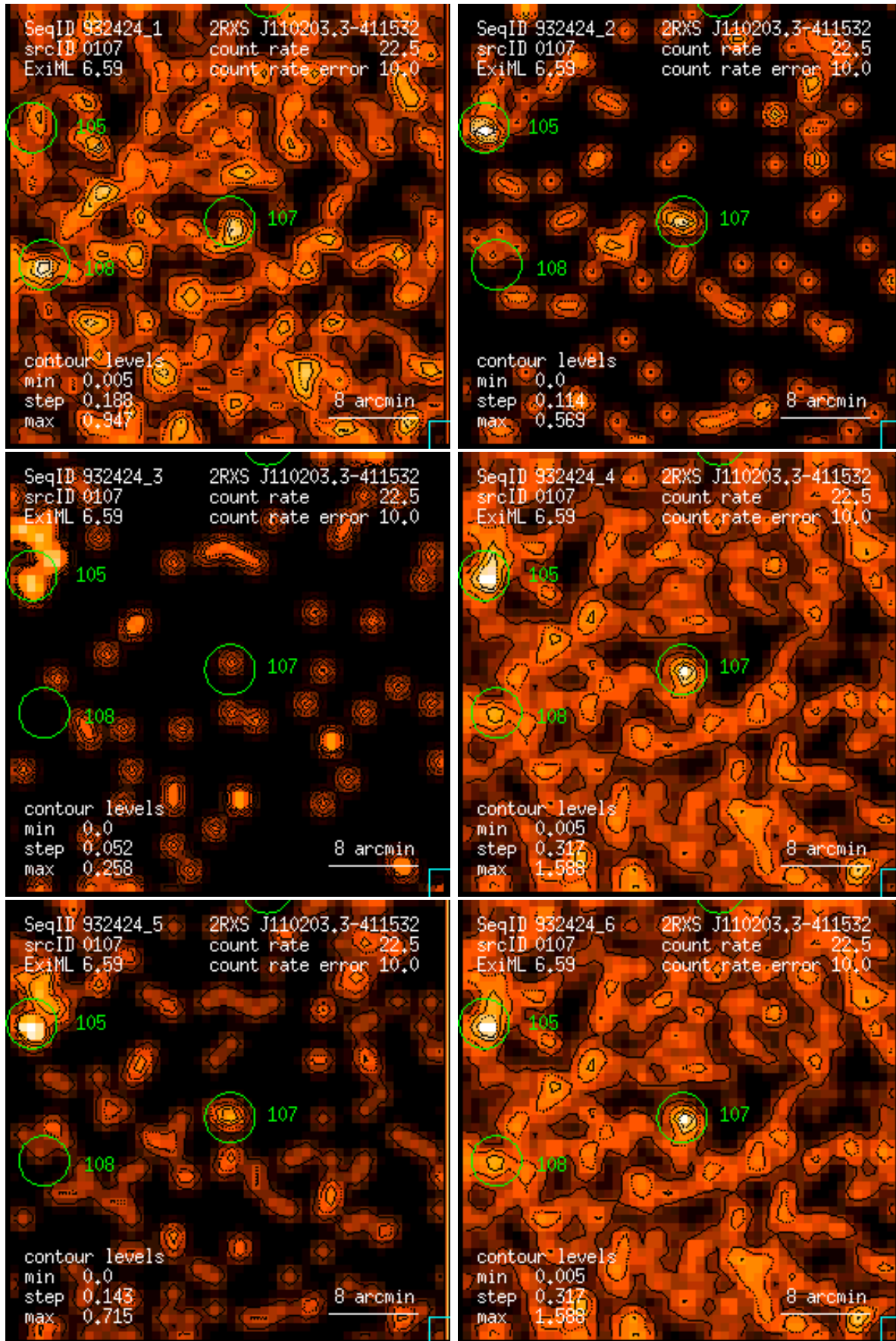
Figure 107: RASS 932424: detection 0107: band rate images, Gaussian filter: (1) PSPC channels 11 – 41, (2) 52 – 90, (3) 91 – 201, (4) 11 – 235, (5) 52 – 201, (6) 11 – 201. Broad band rates in counts/ks. Band rate contour levels in counts/ks/arcmin 2 .
