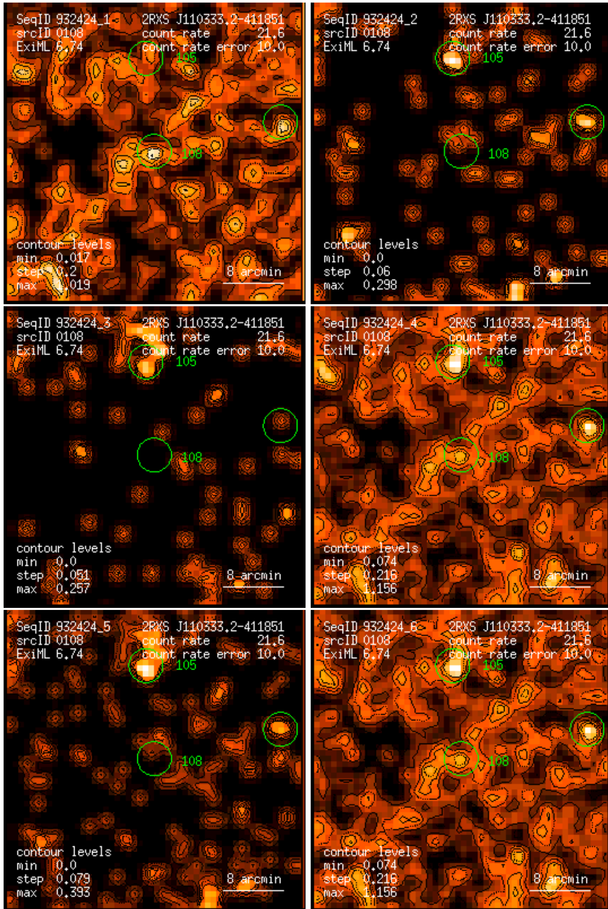
Figure 108: RASS 932424: detection 0108: band rate images, Gaussian filter: (1) PSPC channels 11 – 41, (2) 52 – 90, (3) 91 – 201, (4) 11 – 235, (5) 52 – 201, (6) 11 – 201. Broad band rates in counts/ks. Band rate contour levels in counts/ks/arcmin 2 .
