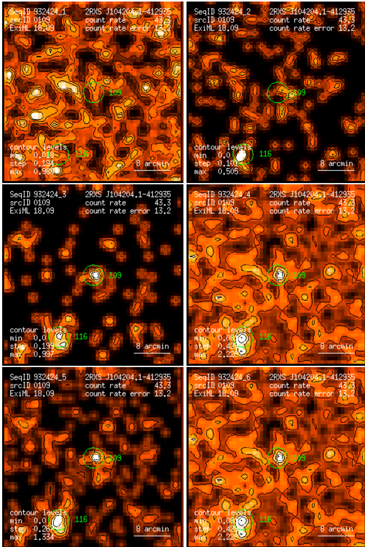
Figure 109: RASS 932424: detection 0109: band rate images, Gaussian filter: (1) PSPC channels 11 – 41, (2) 52 – 90, (3) 91 – 201, (4) 11 – 235, (5) 52 – 201, (6) 11 – 201. Broad band rates in counts/ks. Band rate contour levels in counts/ks/arcmin 2 .
