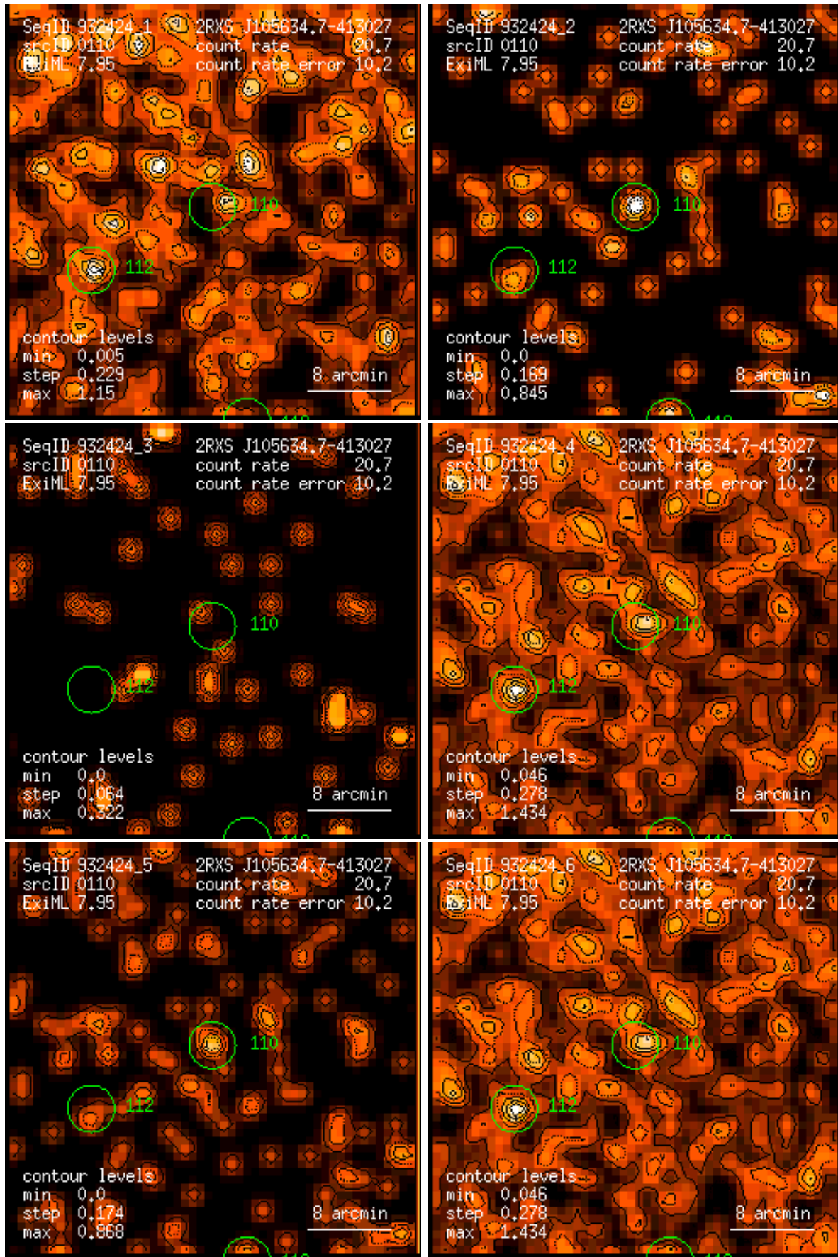
Figure 110: RASS 932424: detection 0110: band rate images, Gaussian filter: (1) PSPC channels 11 – 41, (2) 52 – 90, (3) 91 – 201, (4) 11 – 235, (5) 52 – 201, (6) 11 – 201. Broad band rates in counts/ks. Band rate contour levels in counts/ks/arcmin 2 .
