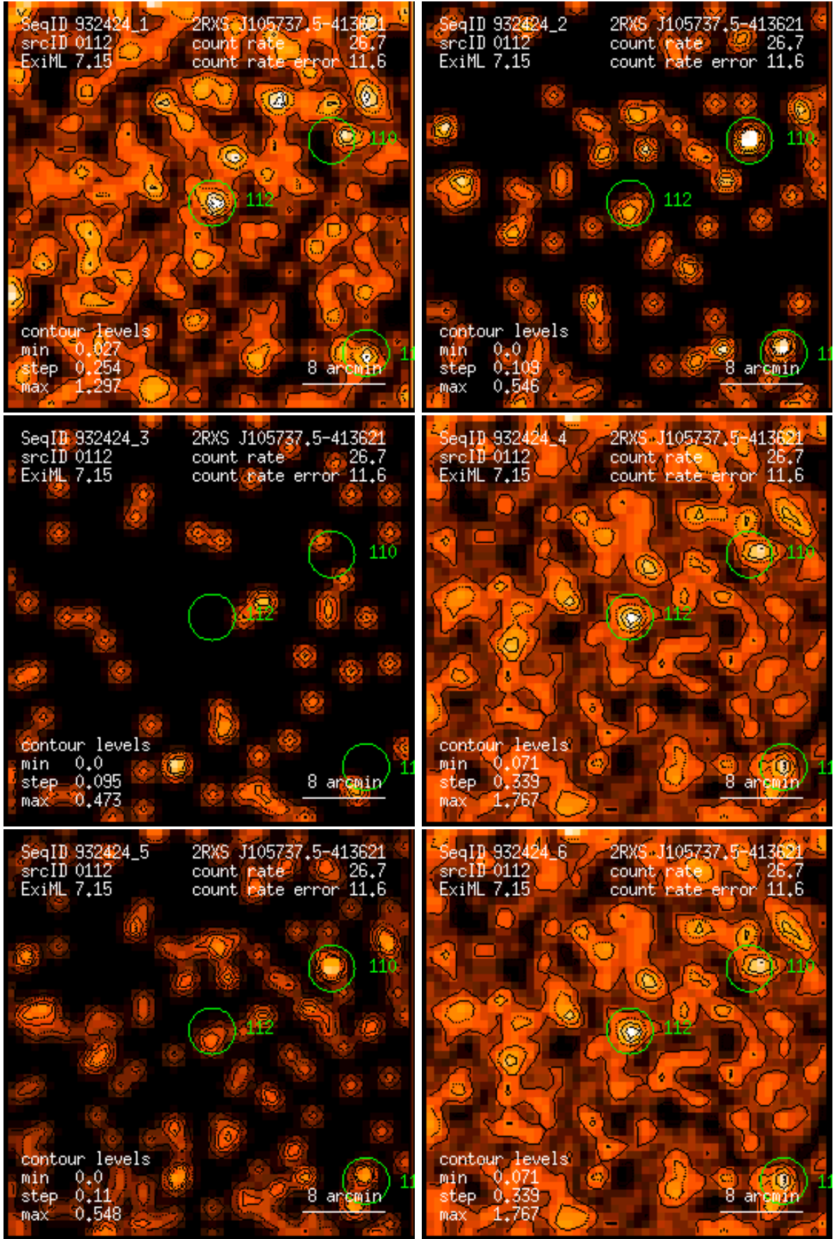
Figure 112: RASS 932424: detection 0112: band rate images, Gaussian filter: (1) PSPC channels 11 – 41, (2) 52 – 90, (3) 91 – 201, (4) 11 – 235, (5) 52 – 201, (6) 11 – 201. Broad band rates in counts/ks. Band rate contour levels in counts/ks/arcmin 2 .
