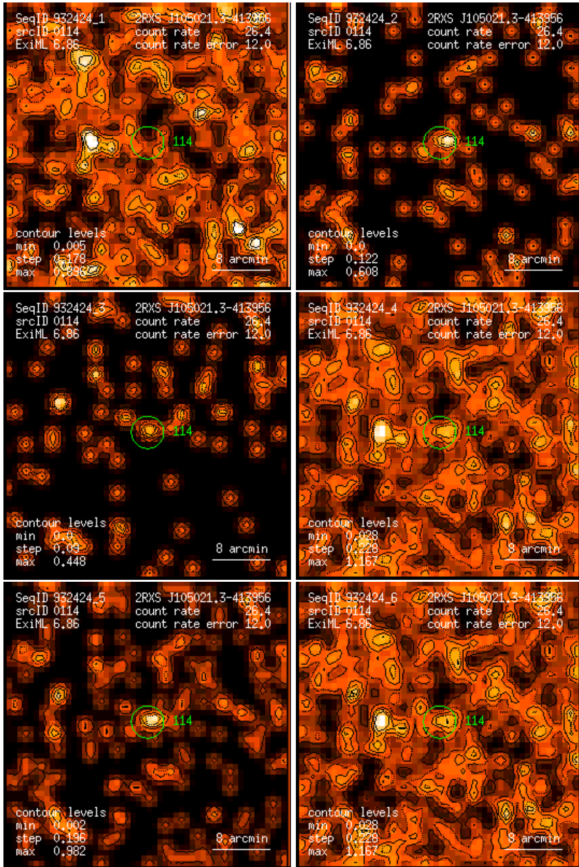
Figure 114: RASS 932424: detection 0114: band rate images, Gaussian filter: (1) PSPC channels 11 – 41, (2) 52 – 90, (3) 91 – 201, (4) 11 – 235, (5) 52 – 201, (6) 11 – 201. Broad band rates in counts/ks. Band rate contour levels in counts/ks/arcmin 2 .
