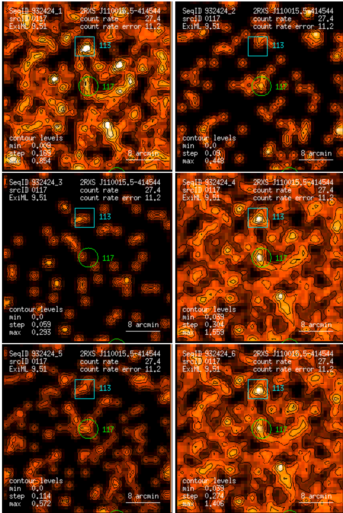
Figure 117: RASS 932424: detection 0117: band rate images, Gaussian filter: (1) PSPC channels 11 – 41, (2) 52 – 90, (3) 91 – 201, (4) 11 – 235, (5) 52 – 201, (6) 11 – 201. Broad band rates in counts/ks. Band rate contour levels in counts/ks/arcmin 2 .
