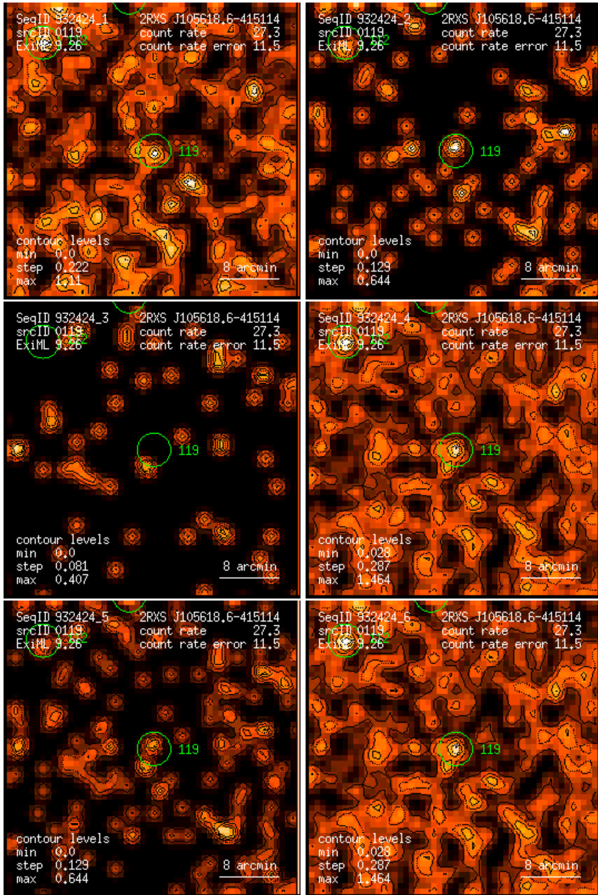
Figure 119: RASS 932424: detection 0119: band rate images, Gaussian filter: (1) PSPC channels 11 – 41, (2) 52 – 90, (3) 91 – 201, (4) 11 – 235, (5) 52 – 201, (6) 11 – 201. Broad band rates in counts/ks. Band rate contour levels in counts/ks/arcmin 2 .
