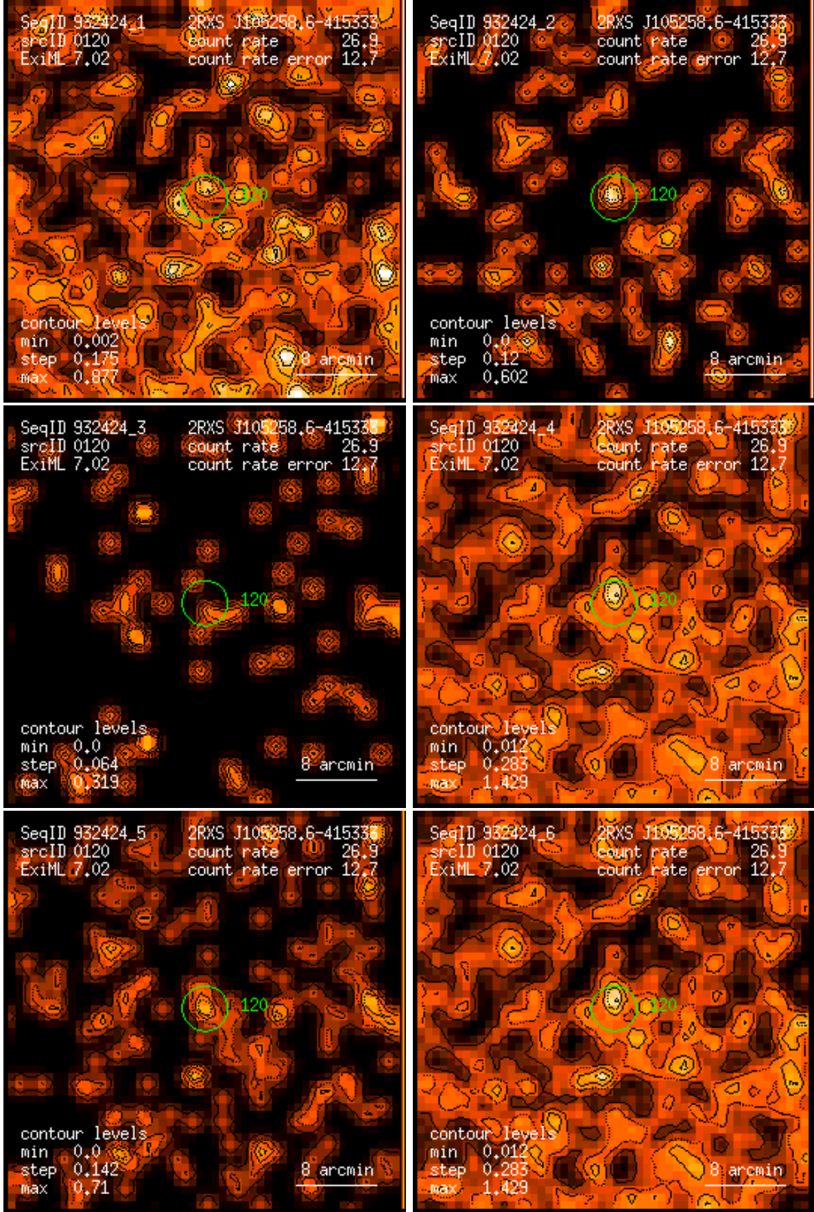
Figure 120: RASS 932424: detection 0120: band rate images, Gaussian filter: (1) PSPC channels 11 – 41, (2) 52 – 90, (3) 91 – 201, (4) 11 – 235, (5) 52 – 201, (6) 11 – 201. Broad band rates in counts/ks. Band rate contour levels in counts/ks/arcmin 2 .
