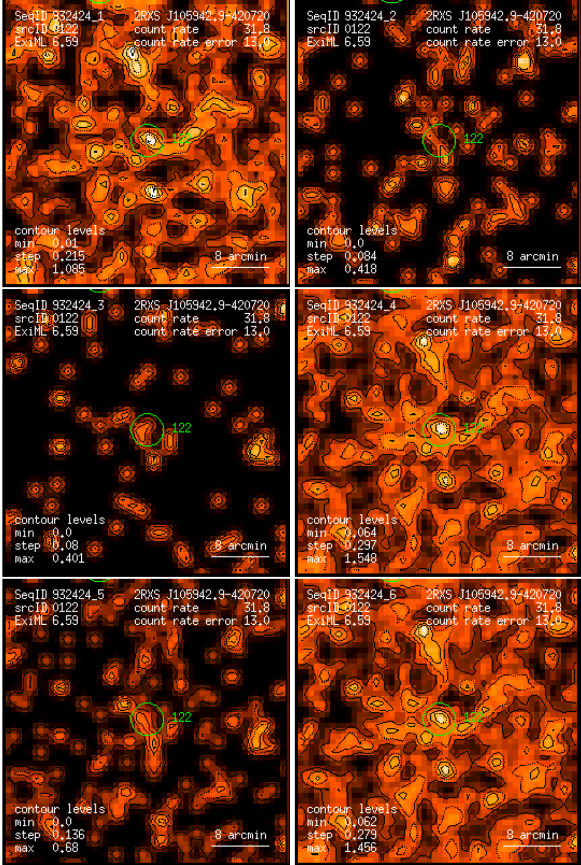
Figure 122: RASS 932424: detection 0122: band rate images, Gaussian filter: (1) PSPC channels 11 – 41, (2) 52 – 90, (3) 91 – 201, (4) 11 – 235, (5) 52 – 201, (6) 11 – 201. Broad band rates in counts/ks. Band rate contour levels in counts/ks/arcmin 2 .
