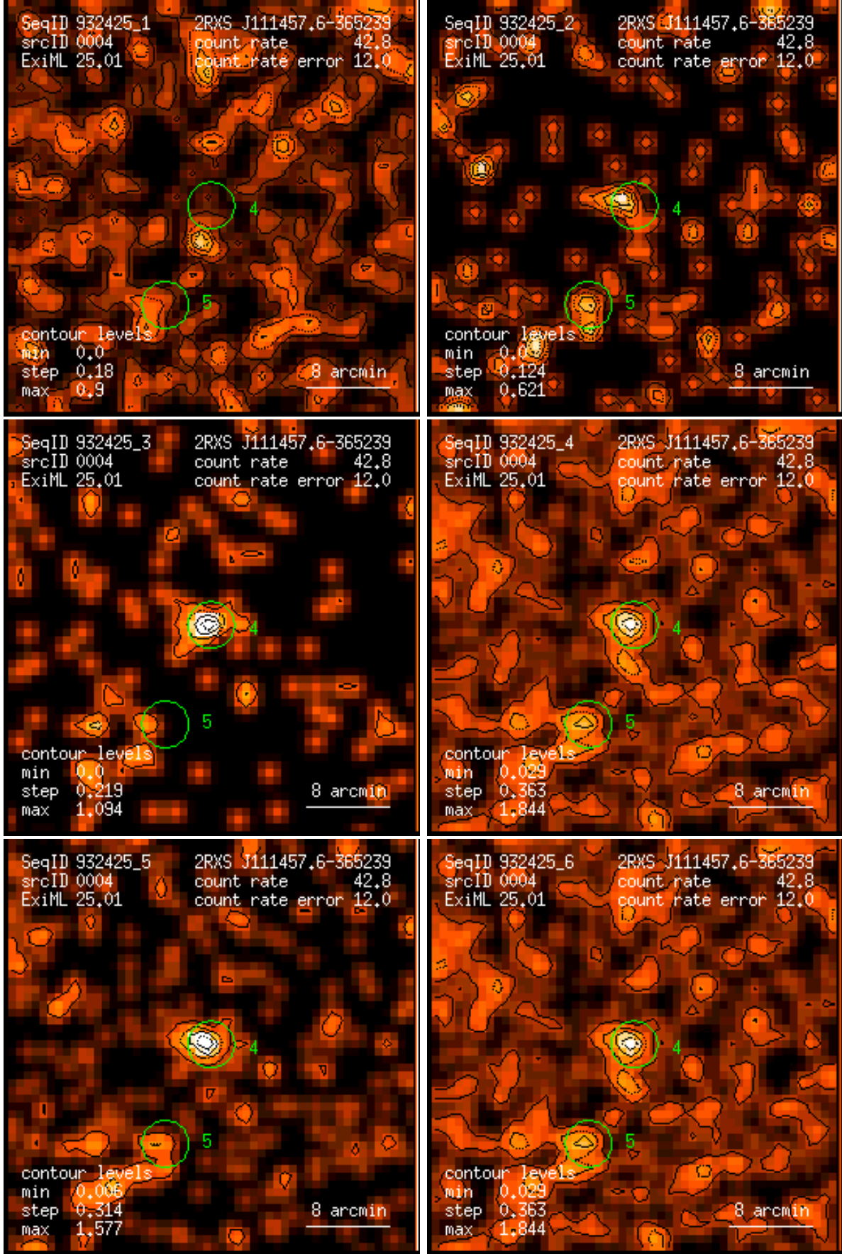
Figure 4: RASS 932425: detection 0004: band rate images, Gaussian filter: (1) PSPC channels 11 – 41, (2) 52 – 90, (3) 91 – 201, (4) 11 – 235, (5) 52 – 201, (6) 11 – 201. Broad band rates in counts/ks. Band rate contour levels in counts/ks/arcmin 2 .
