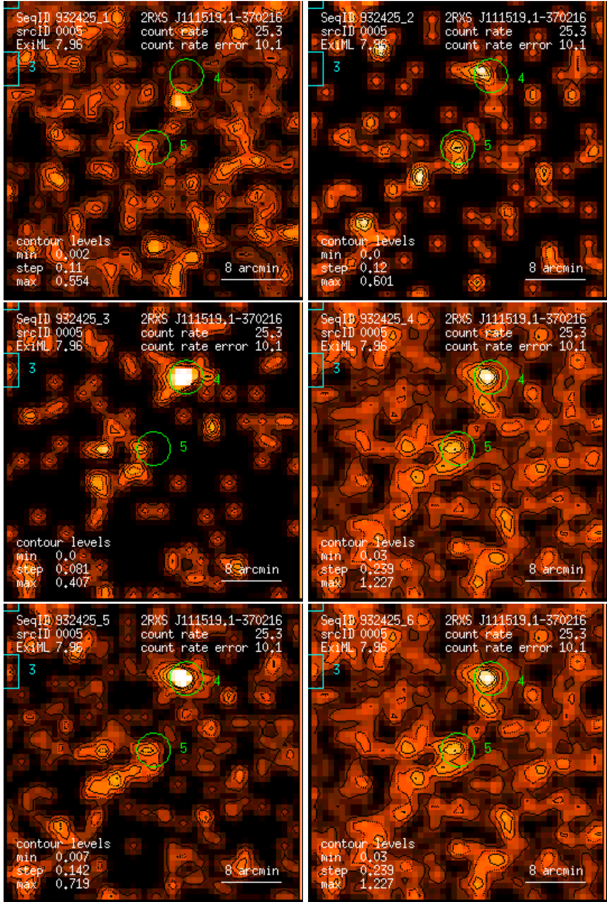
Figure 5: RASS 932425: detection 0005: band rate images, Gaussian filter: (1) PSPC channels 11 – 41, (2) 52 – 90, (3) 91 – 201, (4) 11 – 235, (5) 52 – 201, (6) 11 – 201. Broad band rates in counts/ks. Band rate contour levels in counts/ks/arcmin 2 .
