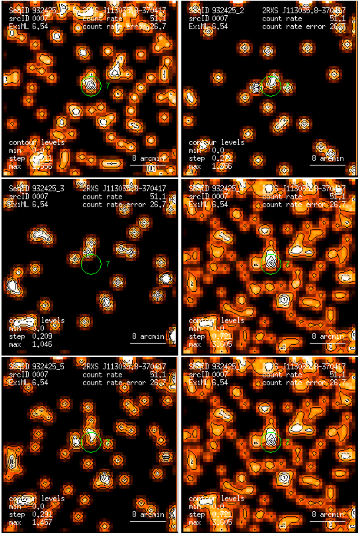
Figure 7: RASS 932425: detection 0007: band rate images, Gaussian filter: (1) PSPC channels 11 – 41, (2) 52 – 90, (3) 91 – 201, (4) 11 – 235, (5) 52 – 201, (6) 11 – 201. Broad band rates in counts/ks. Band rate contour levels in counts/ks/arcmin 2 .
