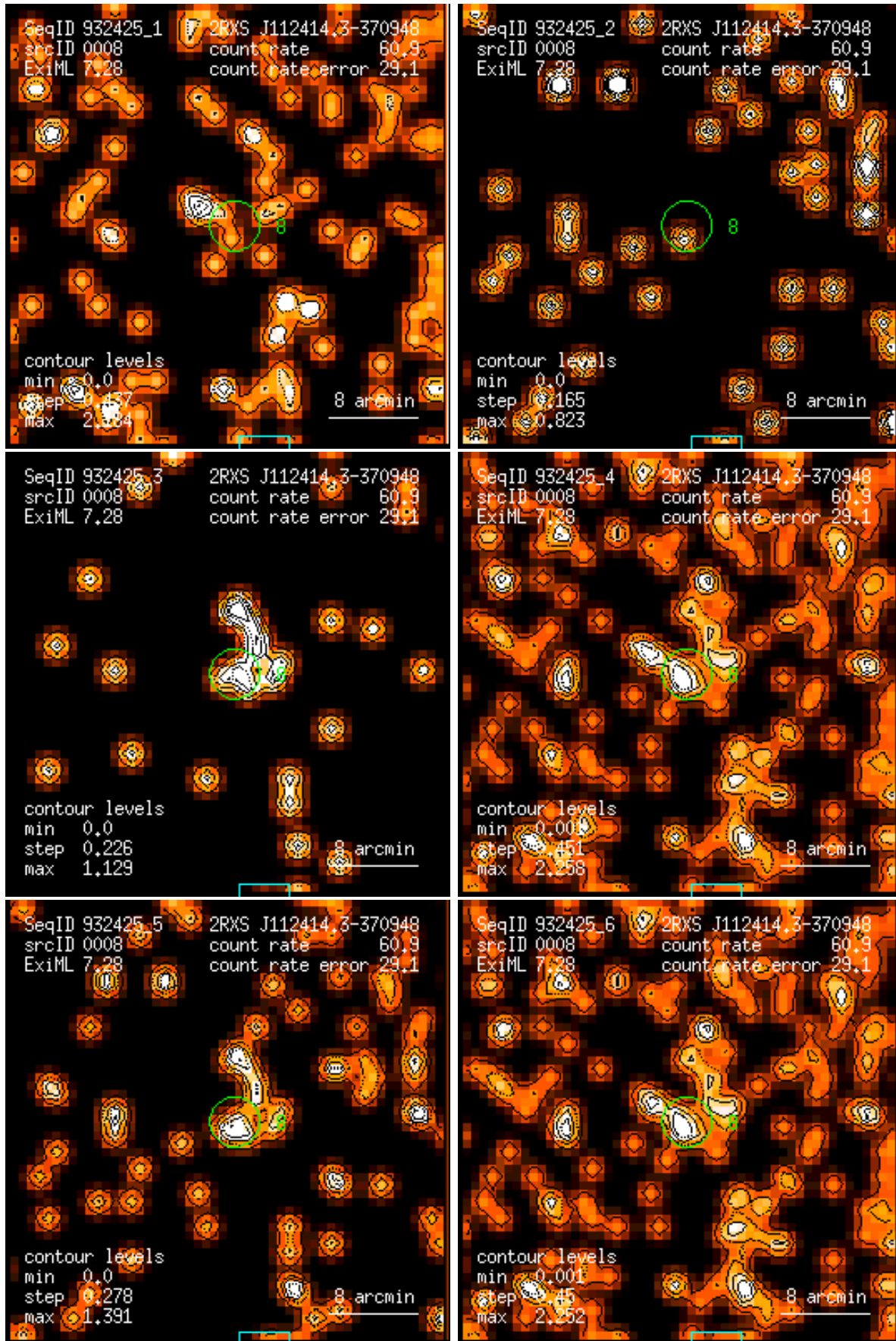
Figure 8: RASS 932425: detection 0008: band rate images, Gaussian filter: (1) PSPC channels 11 – 41, (2) 52 – 90, (3) 91 – 201, (4) 11 – 235, (5) 52 – 201, (6) 11 – 201. Broad band rates in counts/ks. Band rate contour levels in counts/ks/arcmin 2 .
