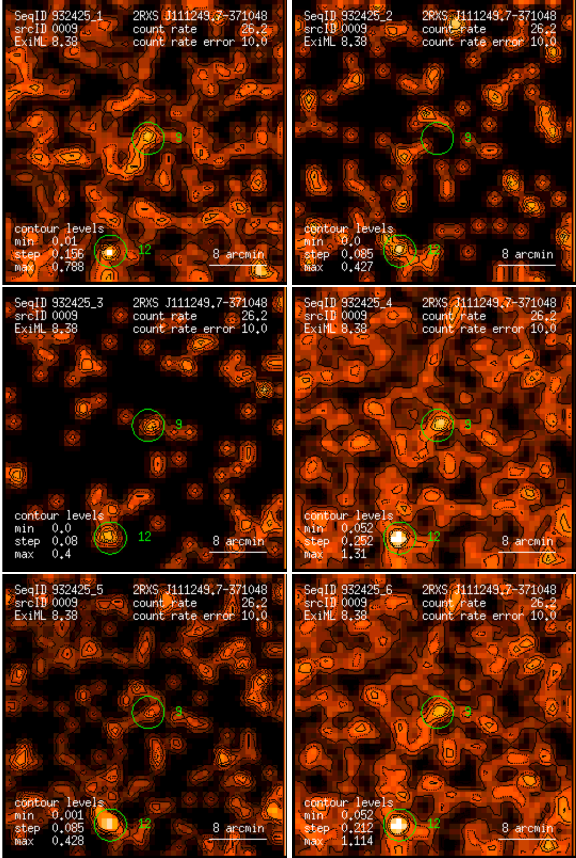
Figure 9: RASS 932425: detection 0009: band rate images, Gaussian filter: (1) PSPC channels 11 – 41, (2) 52 – 90, (3) 91 – 201, (4) 11 – 235, (5) 52 – 201, (6) 11 – 201. Broad band rates in counts/ks. Band rate contour levels in counts/ks/arcmin 2 .
