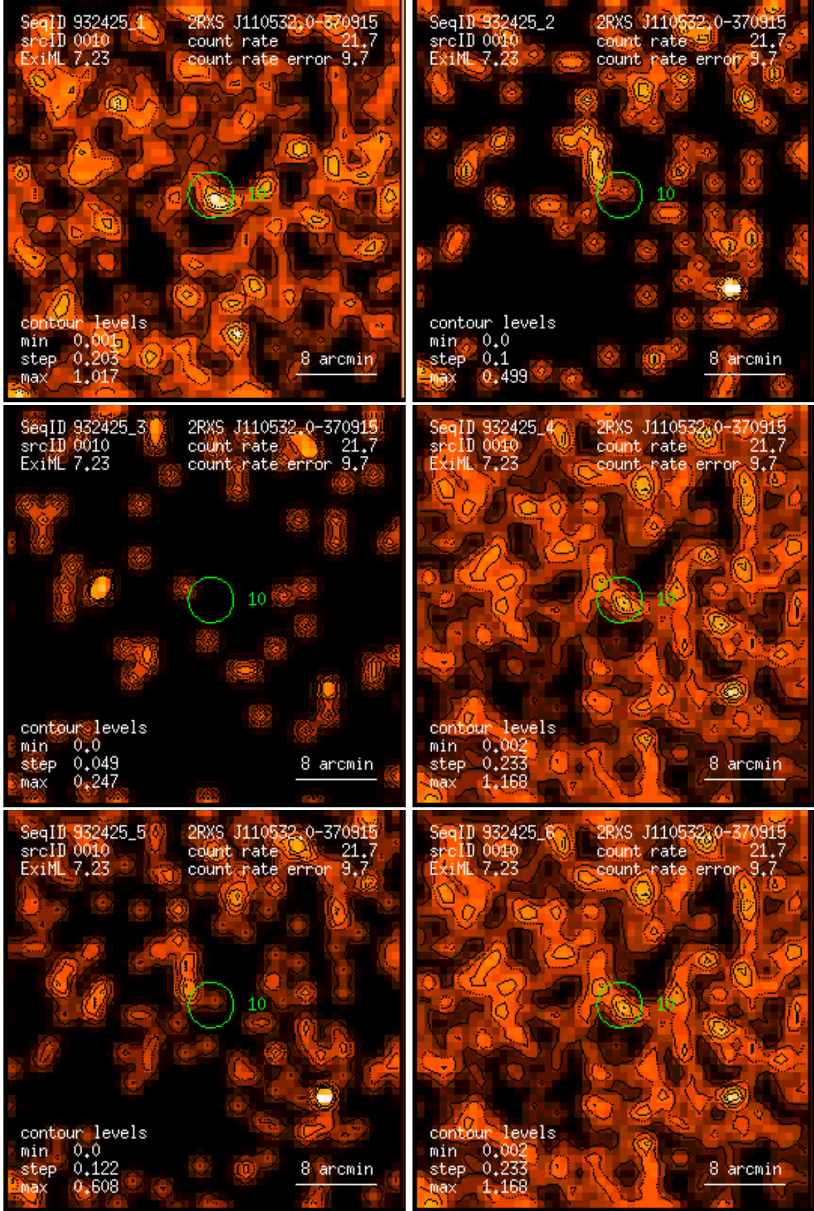
Figure 10: RASS 932425: detection 0010: band rate images, Gaussian filter: (1) PSPC channels 11 – 41, (2) 52 – 90, (3) 91 – 201, (4) 11 – 235, (5) 52 – 201, (6) 11 – 201. Broad band rates in counts/ks. Band rate contour levels in counts/ks/arcmin 2 .
