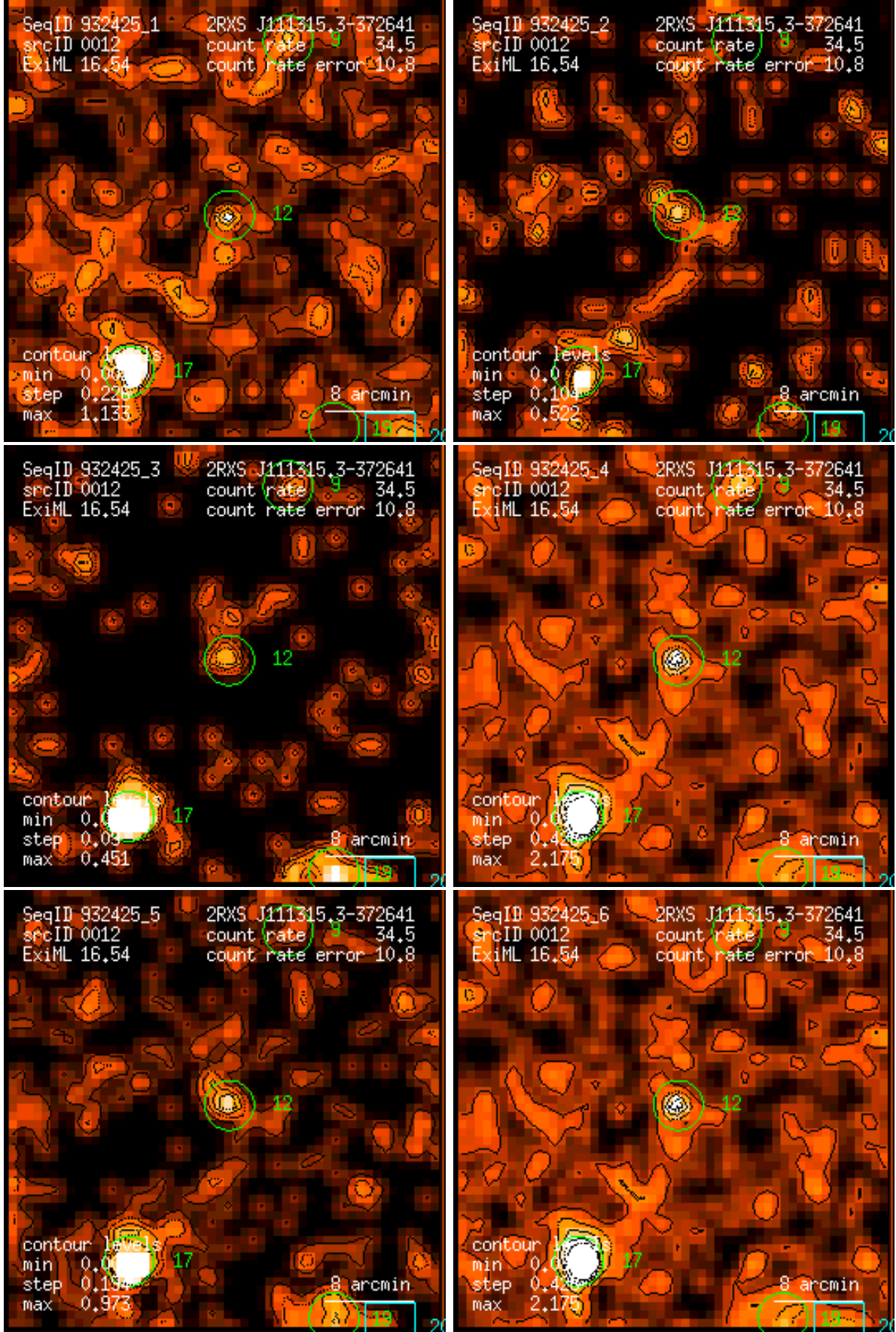
Figure 12: RASS 932425: detection 0012: band rate images, Gaussian filter: (1) PSPC channels 11 – 41, (2) 52 – 90, (3) 91 – 201, (4) 11 – 235, (5) 52 – 201, (6) 11 – 201. Broad band rates in counts/ks. Band rate contour levels in counts/ks/arcmin 2 .
