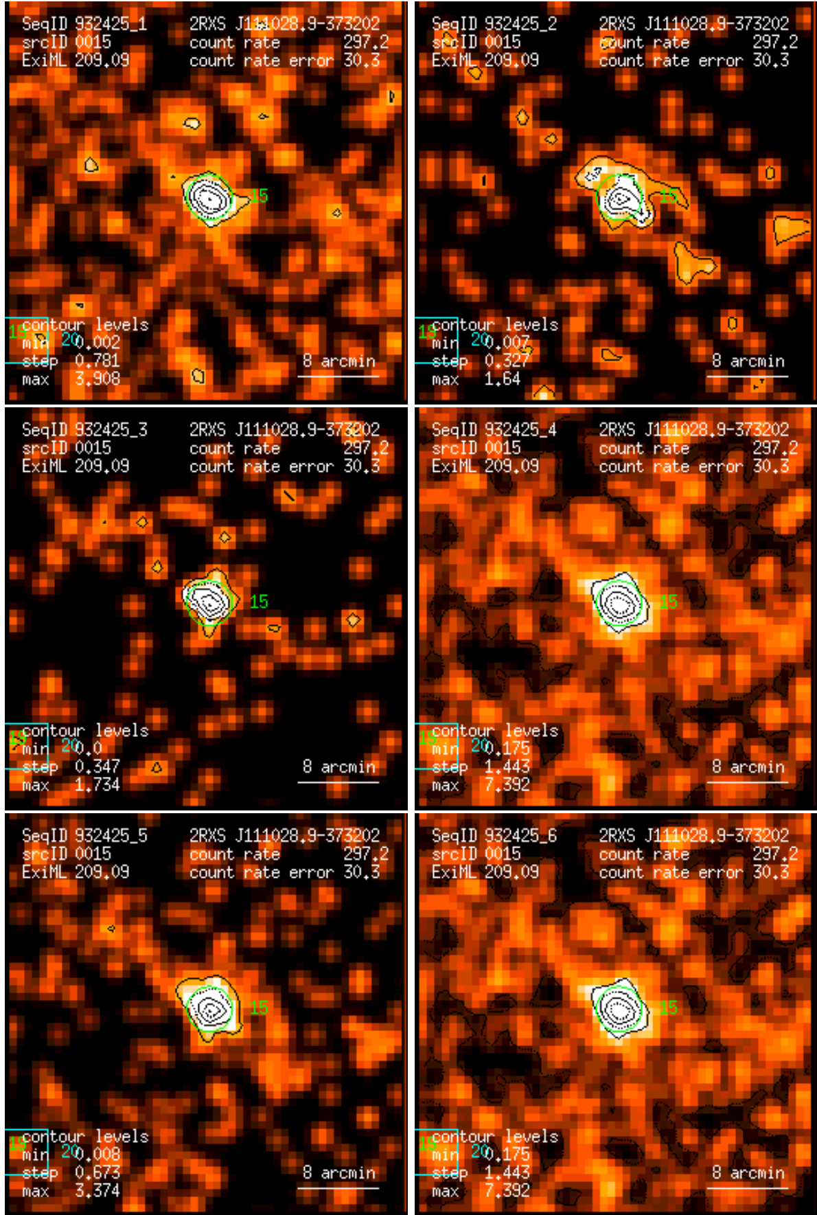
Figure 15: RASS 932425: detection 0015: band rate images, Gaussian filter: (1) PSPC channels 11 – 41, (2) 52 – 90, (3) 91 – 201, (4) 11 – 235, (5) 52 – 201, (6) 11 – 201. Broad band rates in counts/ks. Band rate contour levels in counts/ks/arcmin 2 .
