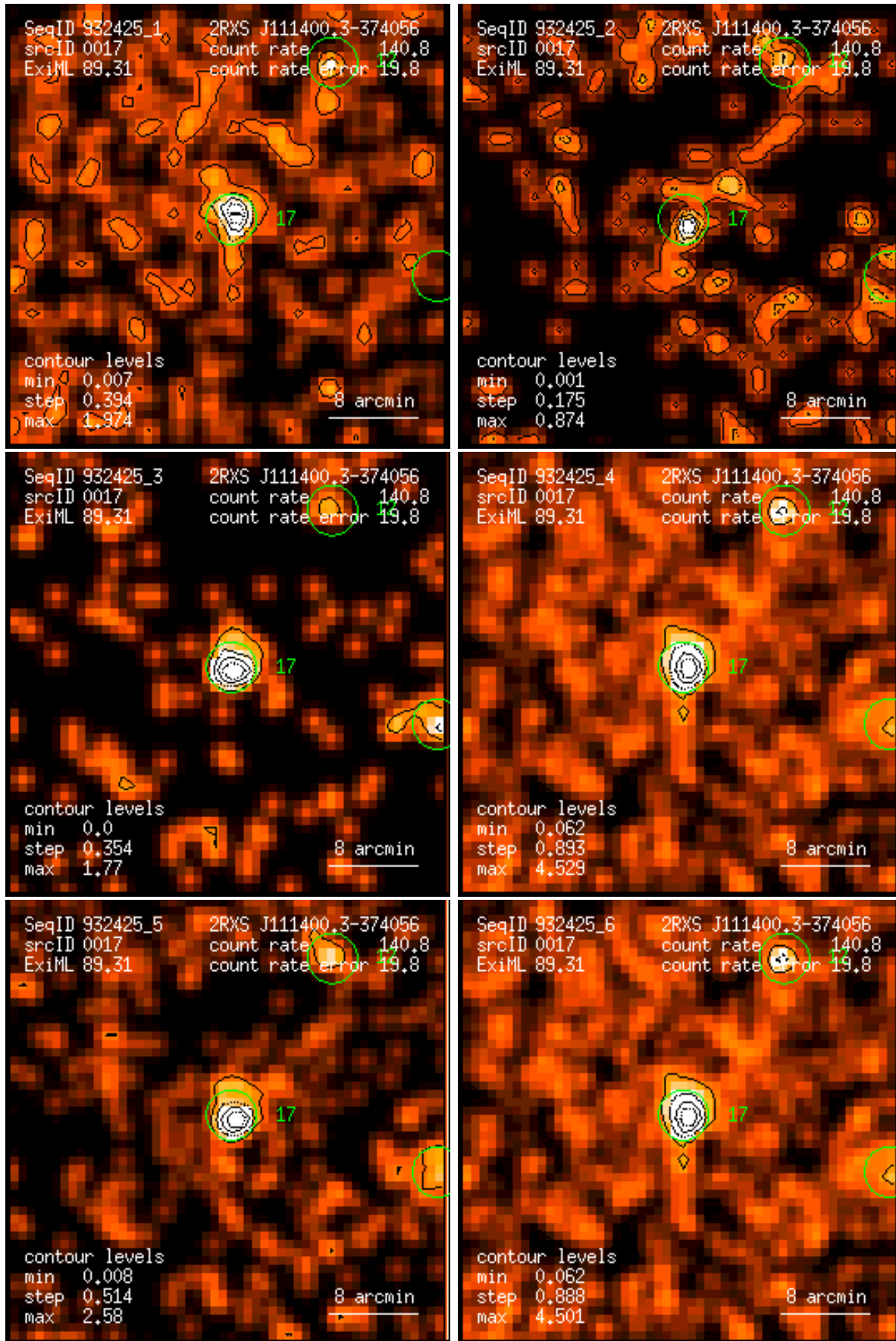
Figure 17: RASS 932425: detection 0017: band rate images, Gaussian filter: (1) PSPC channels 11 – 41, (2) 52 – 90, (3) 91 – 201, (4) 11 – 235, (5) 52 – 201, (6) 11 – 201. Broad band rates in counts/ks. Band rate contour levels in counts/ks/arcmin 2 .
