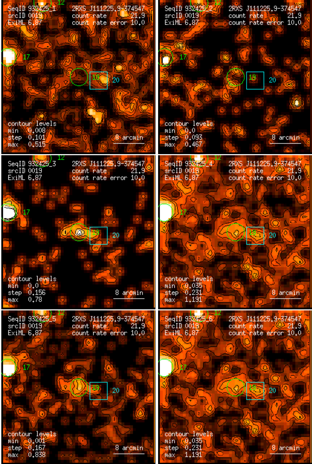
Figure 19: RASS 932425: detection 0019: band rate images, Gaussian filter: (1) PSPC channels 11 – 41, (2) 52 – 90, (3) 91 – 201, (4) 11 – 235, (5) 52 – 201, (6) 11 – 201. Broad band rates in counts/ks. Band rate contour levels in counts/ks/arcmin 2 .
