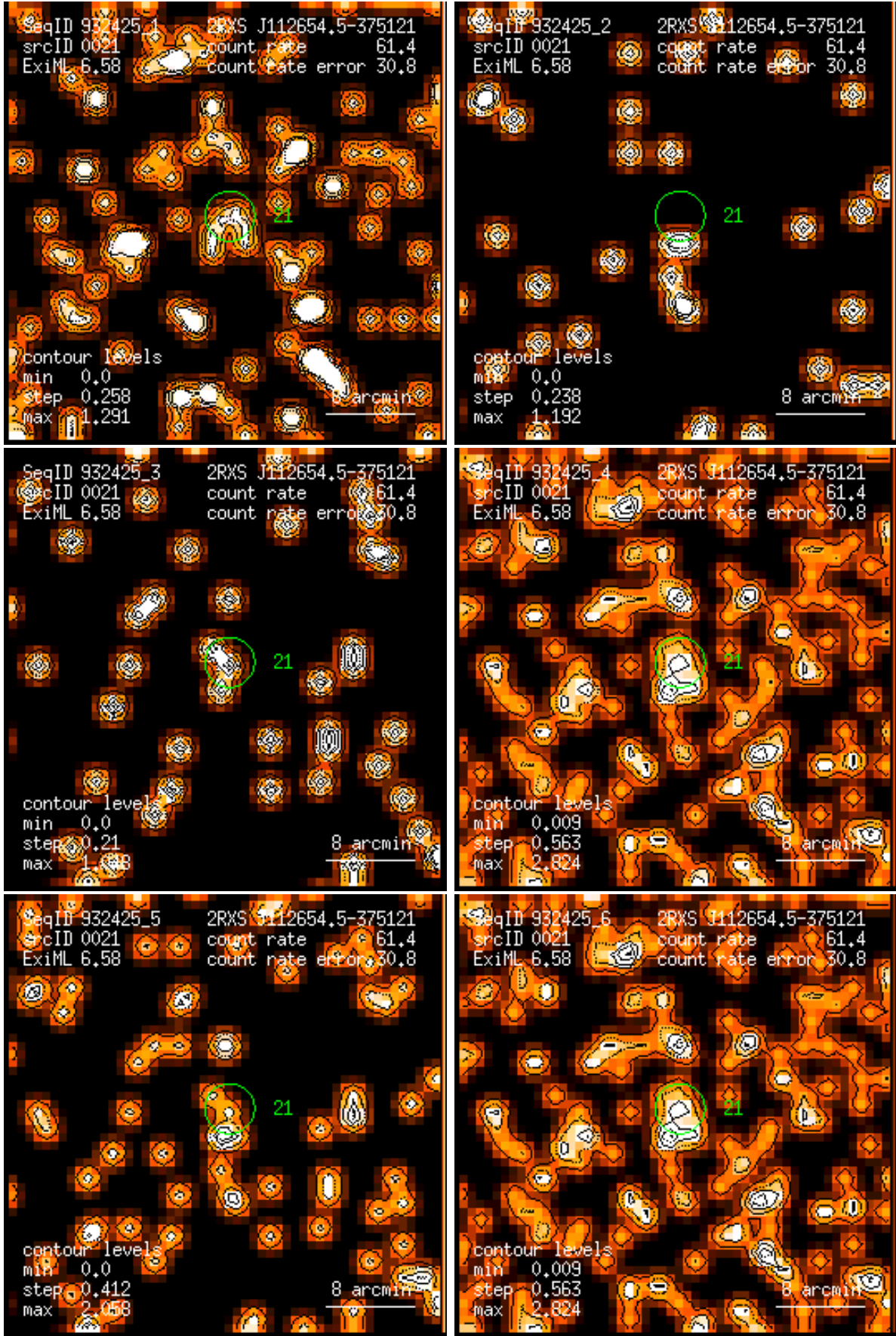
Figure 21: RASS 932425: detection 0021: band rate images, Gaussian filter: (1) PSPC channels 11 – 41, (2) 52 – 90, (3) 91 – 201, (4) 11 – 235, (5) 52 – 201, (6) 11 – 201. Broad band rates in counts/ks. Band rate contour levels in counts/ks/arcmin 2 .
