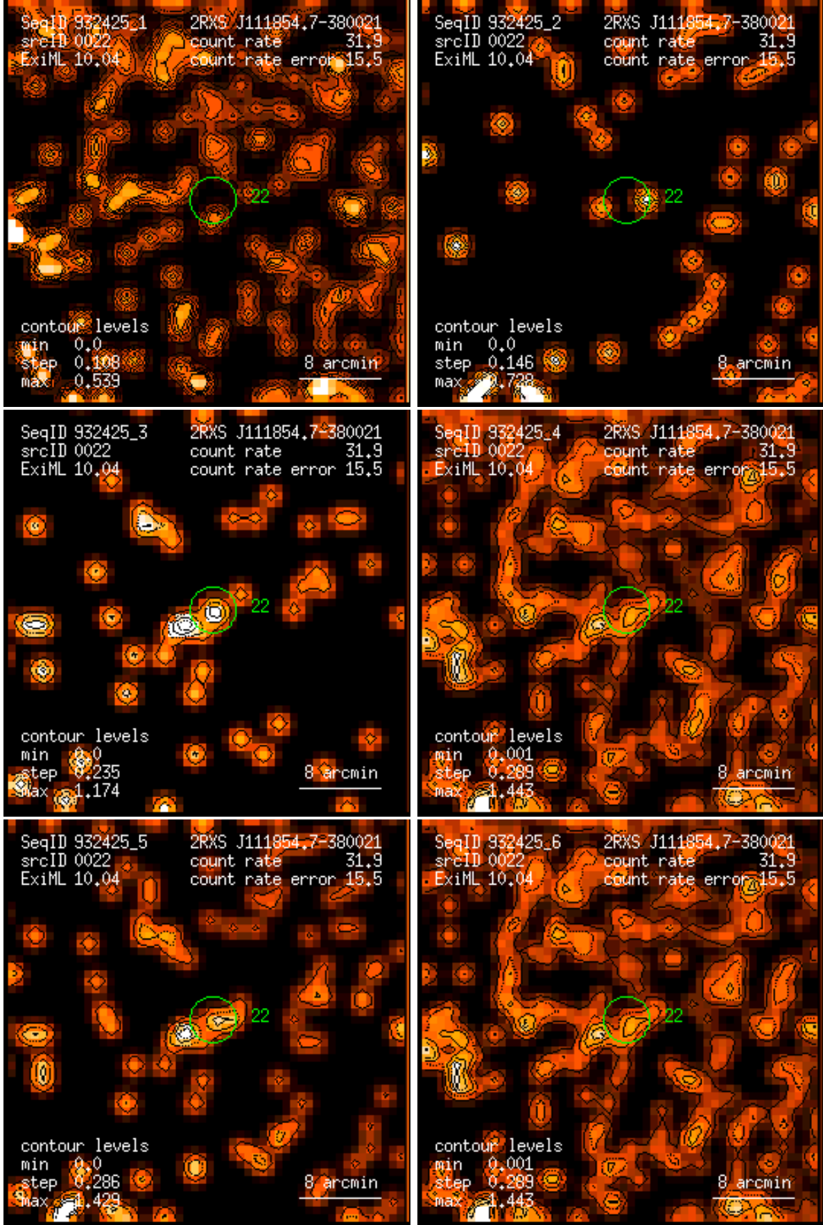
Figure 22: RASS 932425: detection 0022: band rate images, Gaussian filter: (1) PSPC channels 11 – 41, (2) 52 – 90, (3) 91 – 201, (4) 11 – 235, (5) 52 – 201, (6) 11 – 201. Broad band rates in counts/ks. Band rate contour levels in counts/ks/arcmin 2 .
